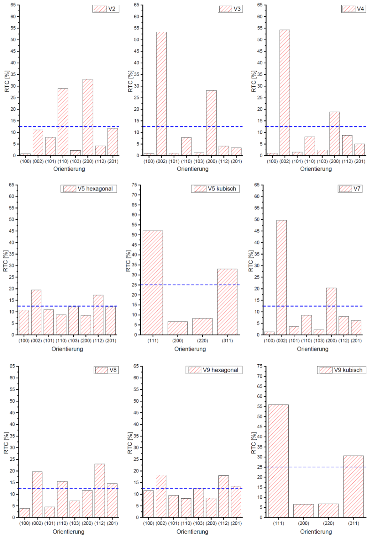
Figure S4. RTC calculations for all experiments, samples prepared on silicon.
