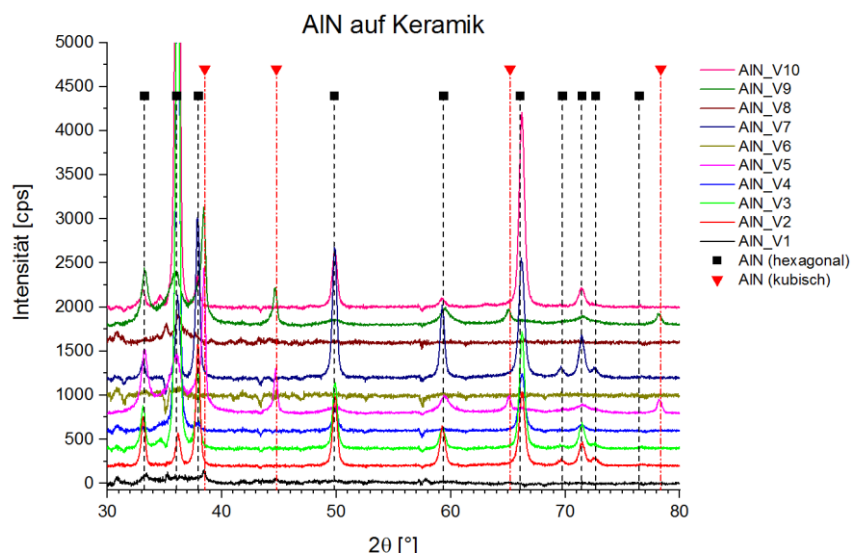
Figure S1. XRD patterns of all samples, sputtered on ceramic.
