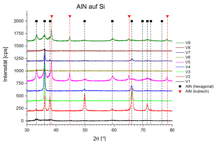
Figure S2. XRD patterns of all samples, sputtered on silicon.
