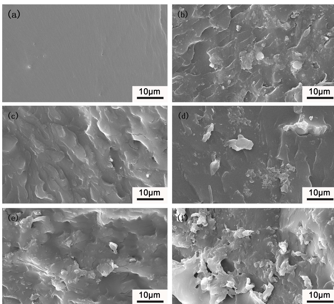
Figure S2. SEM images of cross-section microstructures for smaller magnifications: (a) EP; (b) GO; (c) EGO1; (d) EGO2; (e) EGO3; and (f) EGO4.
