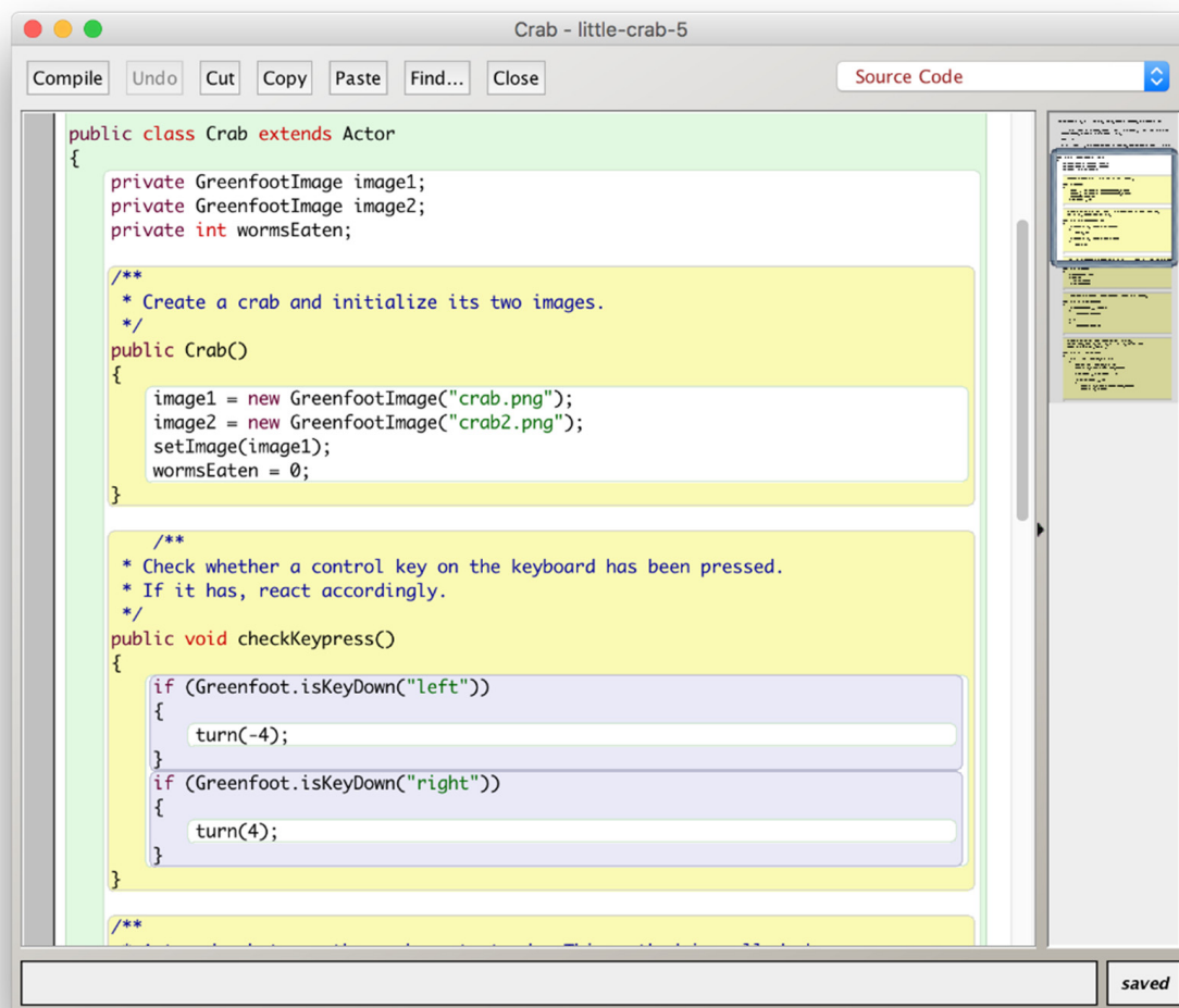
Figure 5. Source code display in the Greenfoot editor. The code is standard Java. The editor uses scope highlighting to illustrate the extent of scopes and their nested structure, such as methods and if-statements.
