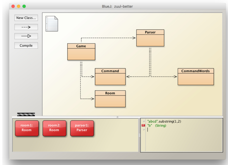
Figure 6. The BlueJ main window. The main part of the window shows a class diagram of the application under development. At the bottom left is the object bench , a place where interactively created objects are displayed. At the bottom right is the Code Pad , an interactive read-eval-print loop that can evaluate single expressions or statements.
