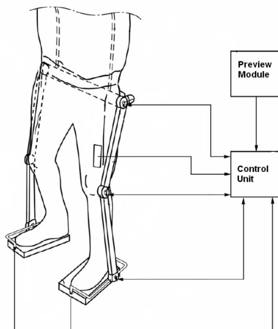
Figure 1. The exoskeleton.
