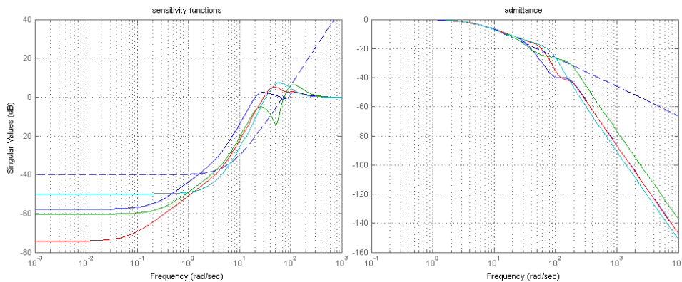
Figure 6. (left) Closed loop output sensitivity functions and (right) admittances, desired and achieved.
