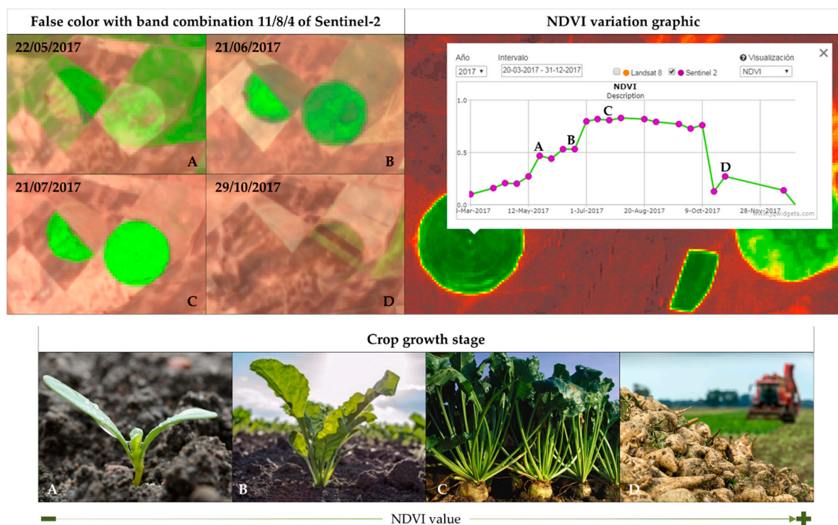
Figure 9. False color images from Sentinel-2 (combination of bands 11, 8 and 4) and a graph of the variation of NDVI TOA values for different dates. This graph represents the growing season profile, including phenological stages, of a sugar beet crop.
