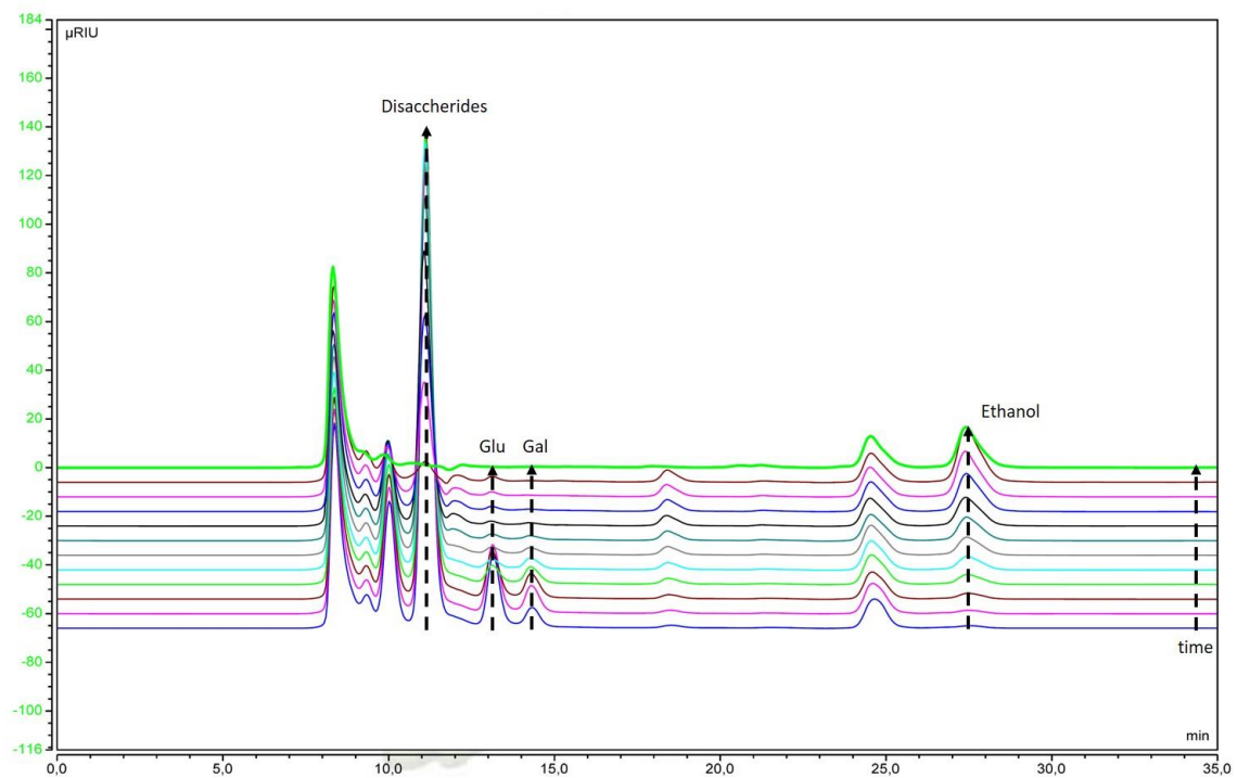
Figure S1. HPLC data of the used pilsner malt extract at different time stages. Increase of ethanol is applicable due to late retention time in the chromatogram. Glucose and Galactose are first, afterwards the disaccharides are consumed by the cells. After consumption of all easy accessible sugars, growth on ethanol starts leading to a decrease in ethanol concentration overnight.
