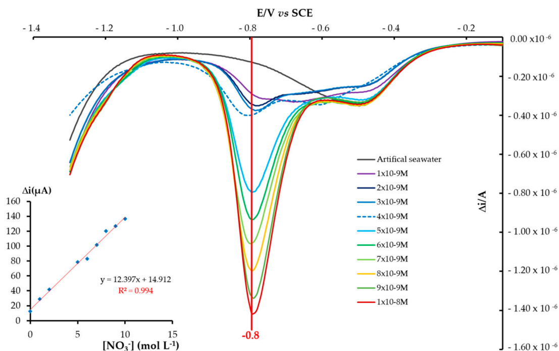
Figure 4. Square wave voltammograms obtained in aerated artificial seawater for successive nitrate ions concentrations on the gold electrode functionalized by in situ metalorganic deposition of silver nanoparticles ( E_{\text{Au/AgNPs}} ). Inset: Calibration plot based on the peak current ( \Delta i ). i vs. [\text{NO}_3^-] and linear regression.
