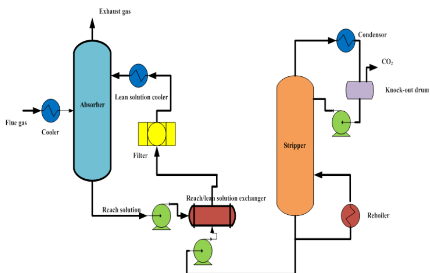
Figure S2. Process flow diagram of the CO 2 recovery unit.
