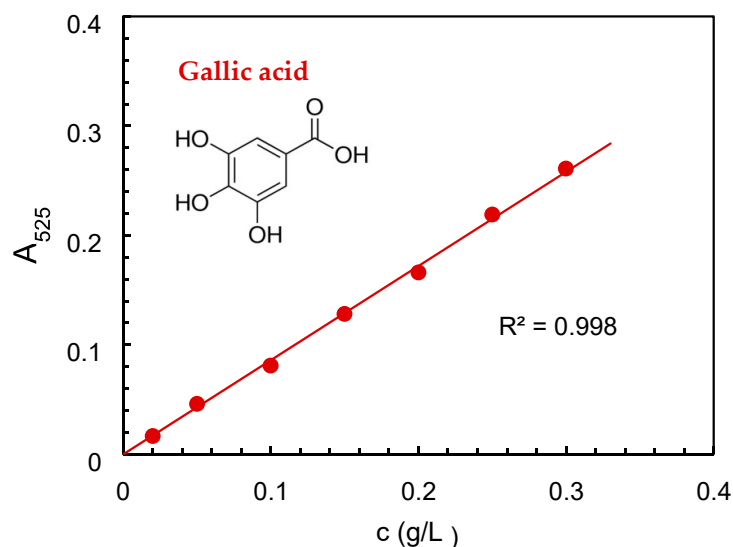
Figure 1. Calibration curves for evaluation of total phenolics.
