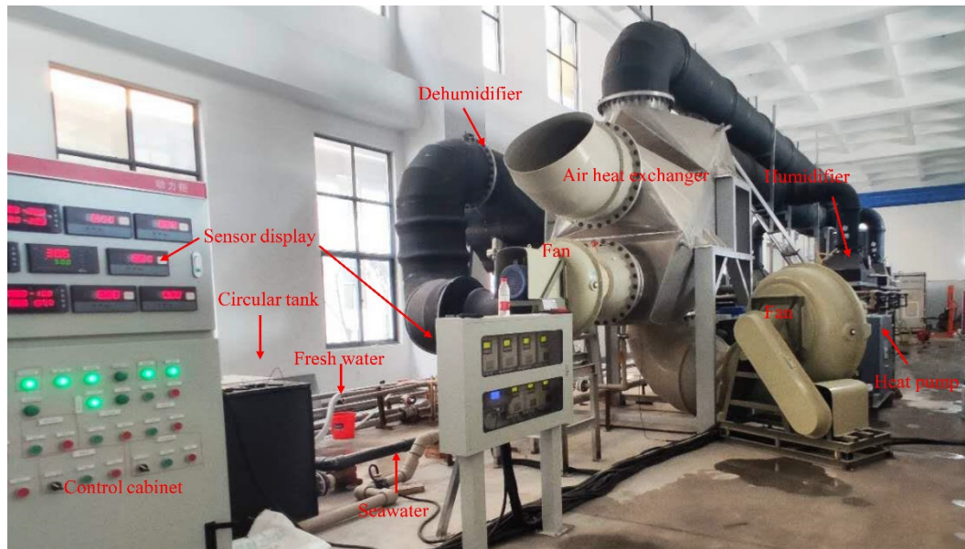
Figure S1. Image of the humidification and dehumidification device.
