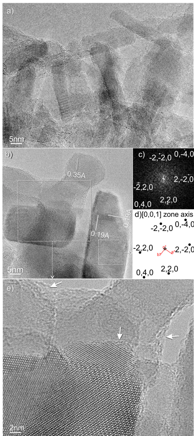
Figure 5. (a,b) HRTEM images of Fe-titanate nanotubes (prepared from Fe(NO_3)_3 0.001 M) after thermal decomposition of C_2H_4 at 750 °C for 1'; (c) experimental FFT image of the nanoparticle selected in (b); which is oriented along the [001] zone axis and (d) the related simulated SAED pattern of the selected area in (d); The arrows in (e) highlight the carbon-decorated TiO_2 nanoparticle edges.
