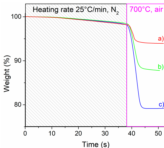
Figure 7. TGA curves obtained from a two-step measurement (heating under N_2 , and oxidation in air at 700 °C) for the Fe-TiTs contacted with C_2H_4 at 750 °C for 1': (a) about 0.4 wt %; (b) 2 wt %, and (c) 3 wt % of Fe, respectively.
