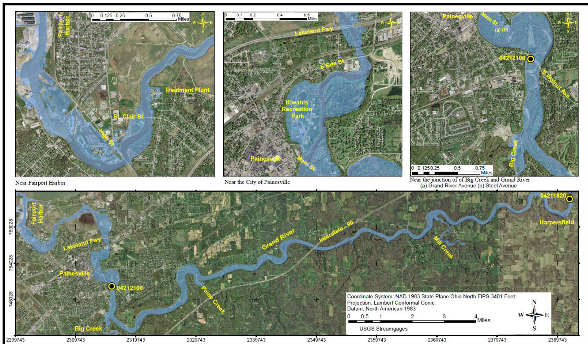
Figure S11 : Flood inundation map along the Grand River, for the stage of 20.00 feet, 615.59 feet NAVD 88 at 04212100 and the stage of 18.62 feet, 751.62 feet NAVD 88 at 04211820
