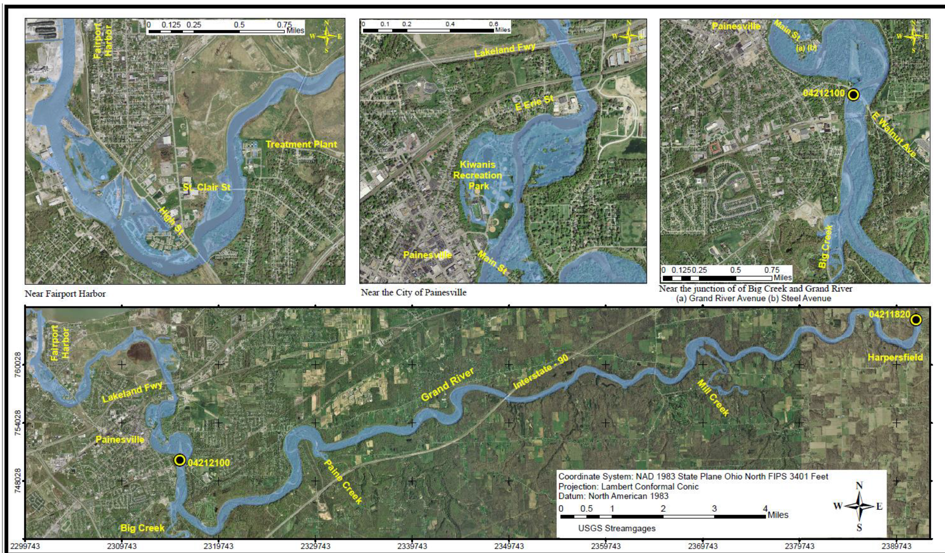
Figure S7 : Flood inundation map along the Grand River, for the stage of 16.00 feet, 611.59 feet NAVD 88 at 04212100 and the stage of 15.35 feet, 748.35 feet NAVD 88 at 04211820
