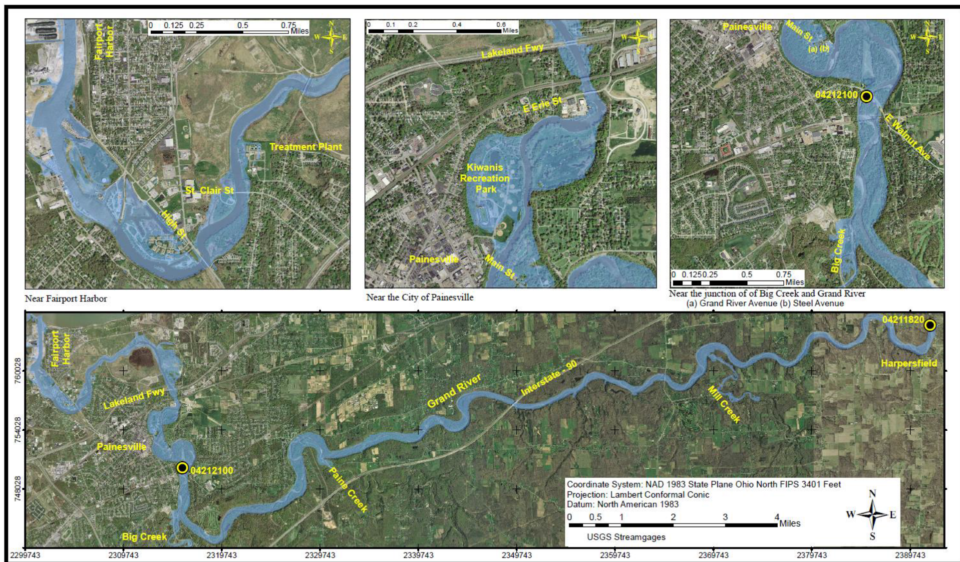
Figure S9 : Flood inundation map along the Grand River, for the stage of 18.00 feet, 613.59 feet NAVD 88 at 04212100 and the stage of 16.96 feet, 749.96 feet NAVD 88 at 04211820
