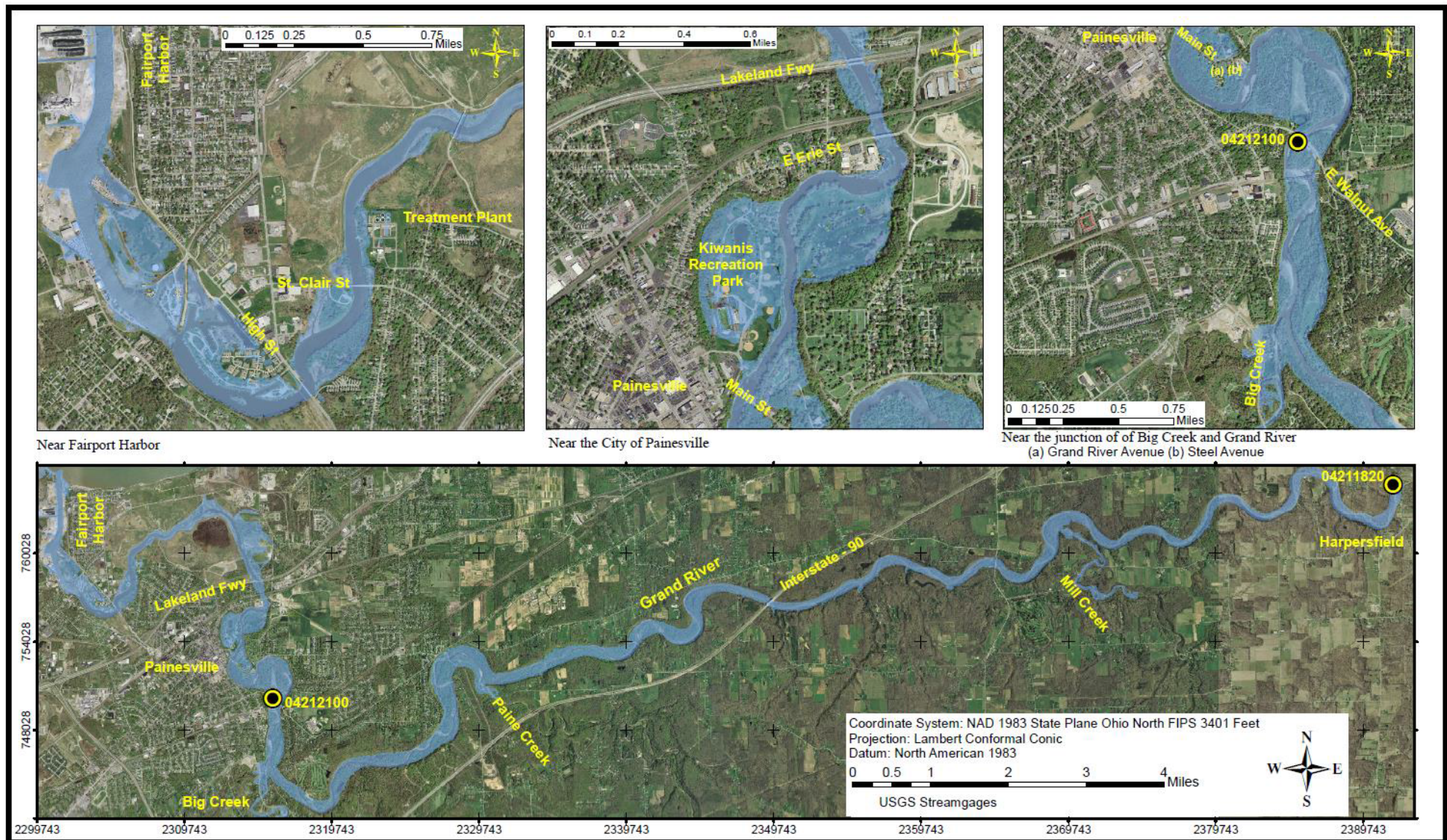
Figure S8 : Flood inundation map along the Grand River, for the stage of 17.00 feet, 612.59 feet NAVD 88 at 04212100 and the stage of 16.15 feet, 749.15 feet NAVD 88 at 04211820
