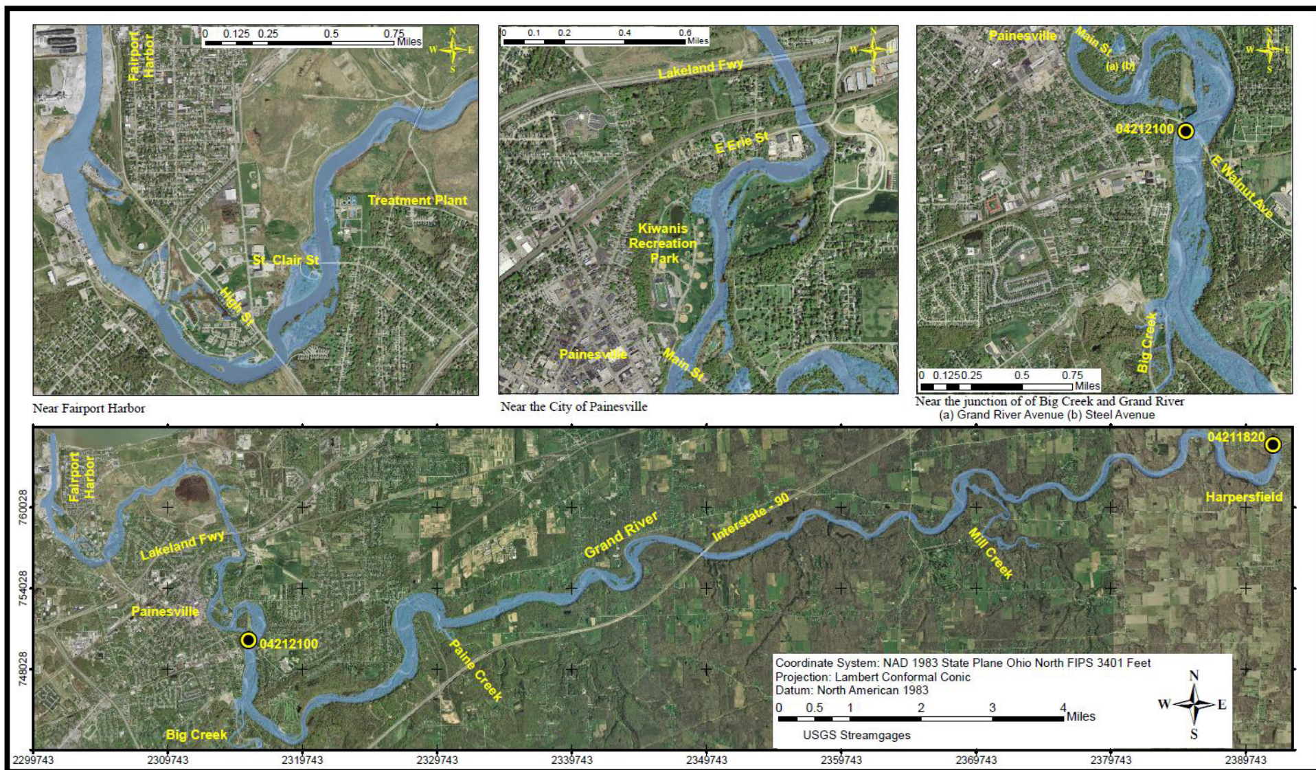
Figure S2 : Flood inundation map along the Grand River, for the stage of 11.00 feet, 606.59 feet NAVD 88 at 04212100 and the stage of 11.07 feet, 744.07 feet NAVD 88 at 04211820
