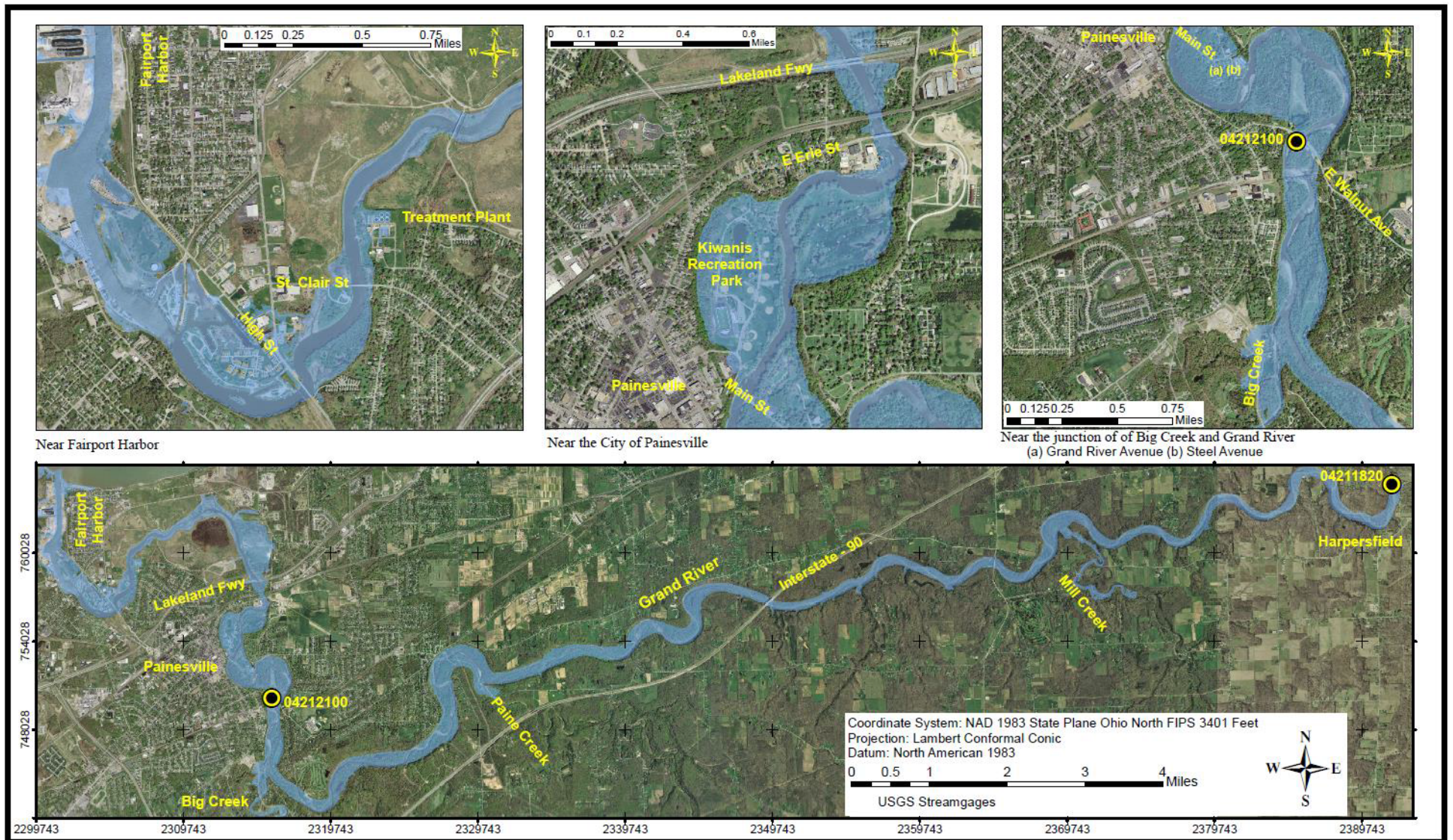
Figure S12 : Flood inundation map along the Grand River, for the stage of 21.00 feet, 616.59 feet NAVD 88 at 04212100 and the stage of 19.42 feet, 752.42 feet NAVD 88 at 04211820
