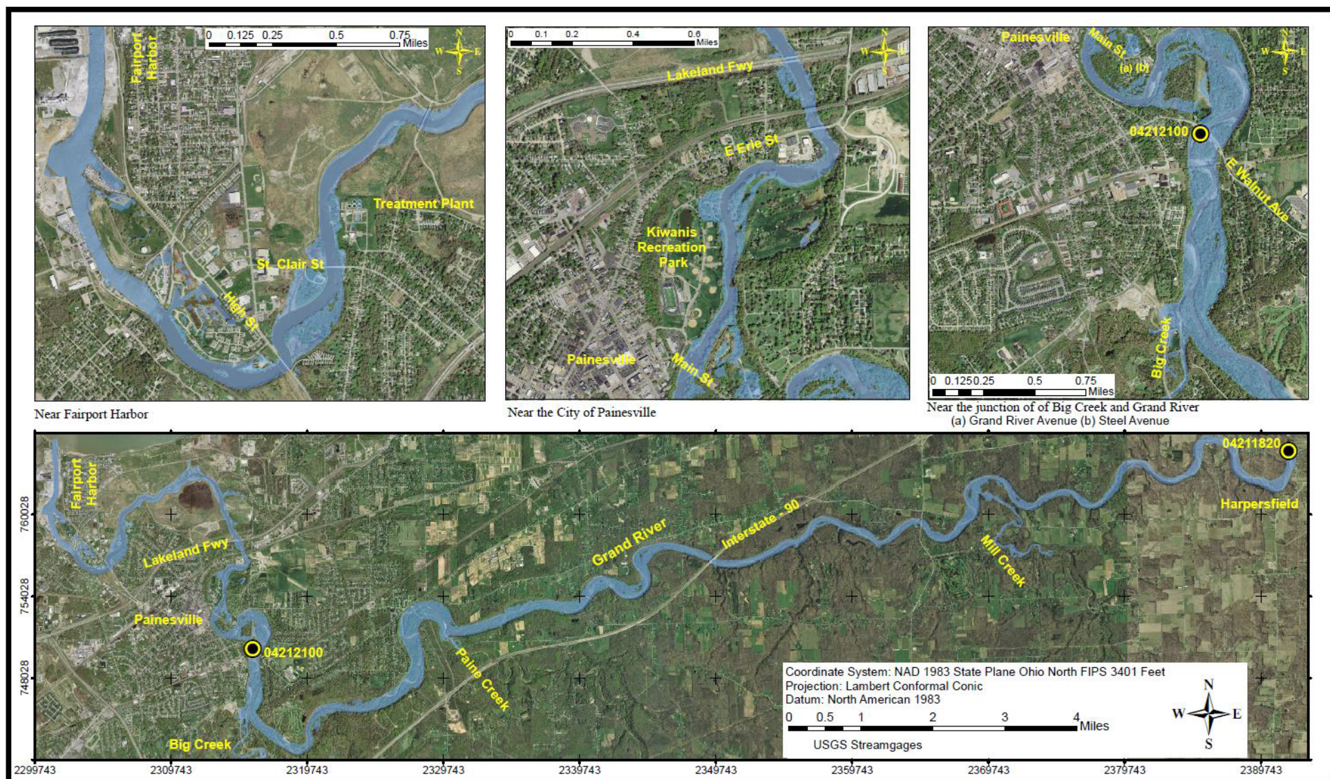
Figure S3 : Flood inundation map along the Grand River, for the stage of 12.00 feet, 607.59 feet NAVD 88 at 04212100 and the stage of 11.99 feet, 744.99 feet NAVD 88 at 04211820
