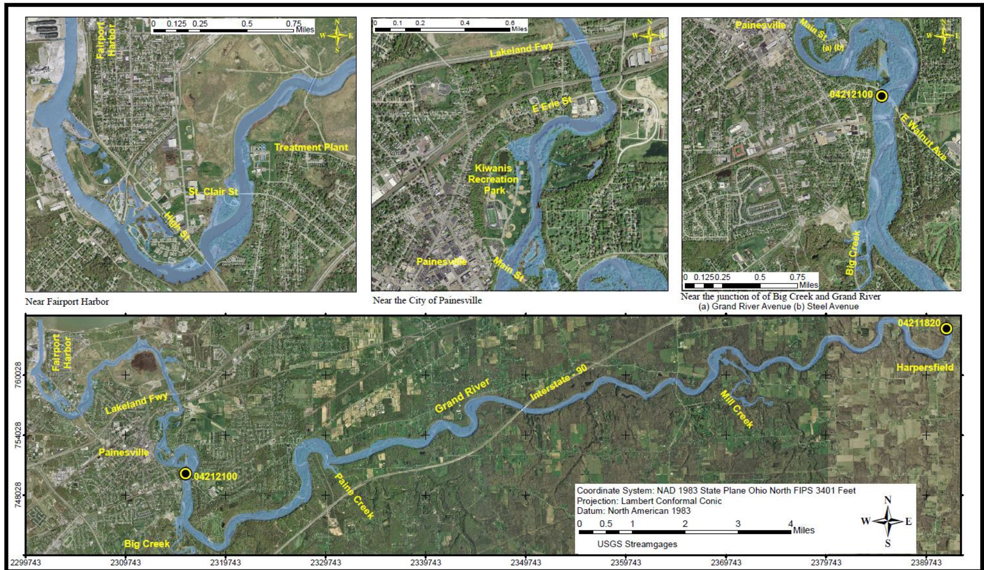
Figure S4 : Flood inundation map along the Grand River, for the stage of 13.00 feet, 608.59 feet NAVD 88 at 04212100 and the stage of 12.86 feet, 745.86 feet NAVD 88 at 04211820
