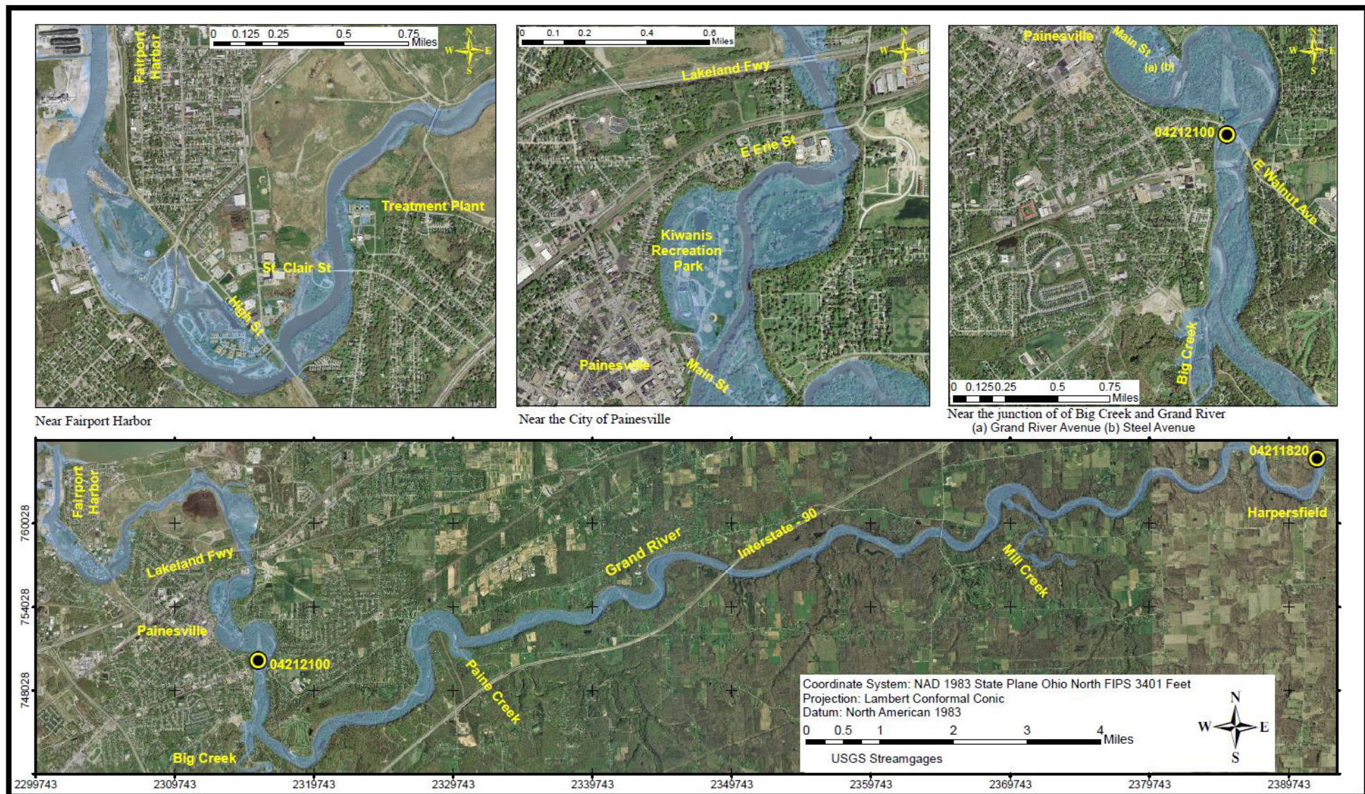
Figure S10 : Flood inundation map along the Grand River, for the stage of 19.35 feet, 614.94 feet NAVD 88 at 04212100 and the stage of 18.10 feet, 751.10 feet NAVD 88 at 04211820
