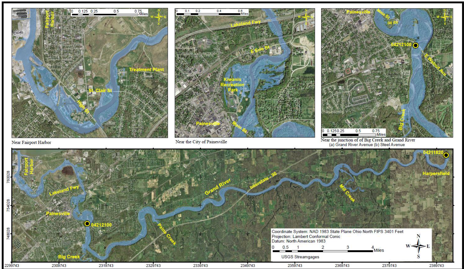
Figure S6 : Flood inundation map along the Grand River, for the stage of 15.00 feet, 610.59 feet NAVD 88 at 04212100 and the stage of 14.53 feet, 747.53 feet NAVD 88 at 04211820
