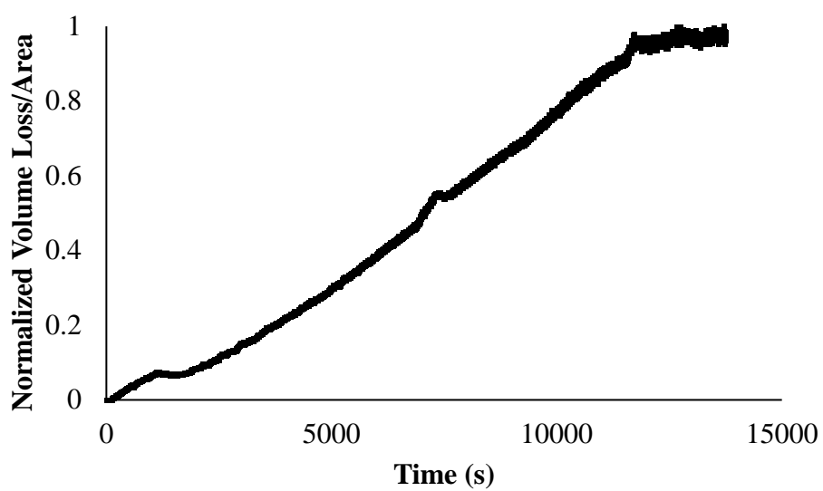
Figure S2: Dynamic volumetric changes in pendant droplets during release of 1-hexanol in MG 57 suspensions in terms of (A) volume of the pendant droplet or (B) volume loss of pendant droplet normalized by the droplet interfacial area and the total volume loss at long times.
