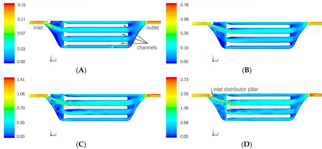
Figure 9. Velocity contours for a plane parallel to the ground ( z = 0.5 mm) for geometry B for different velocity inlets (A) 0.1 m/s, (B) 0.5 m/s, (C) 1.0 m/s and (D) 2.0 m/s.
