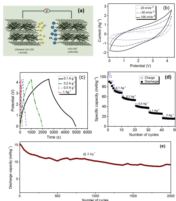
Figure 5. (a) Schematic illustration of the rGO-CNT//lithiated rGO-CNT LIC. (b) CV of the LIC recorded between 0.01–4.3 V voltage window at different scan rates. (c) GCD curves of the LIC. (d) Rate performance of the LIC at different current densities. (e) Cycle performance of the LIC at a current density of 2 \text{Ag}^{-1} for 2000 cycles.
