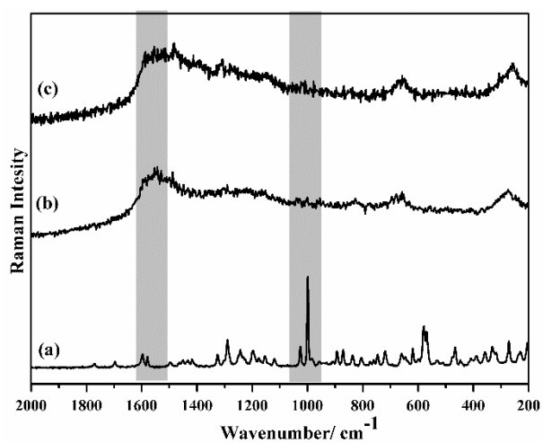
Figure S2. (a) Raman spectra of powdered PG solid and (b) of MNP(102) substrates; (c) control SERS experiment on MNP substrates and using a solution 10^{-4} M in the analyte. Excitation line 633 nm.
