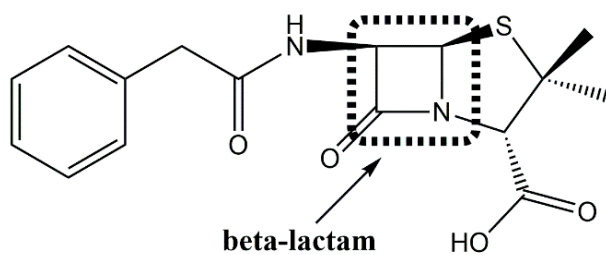
Figure S1. Schematic structure of penicillin G.
