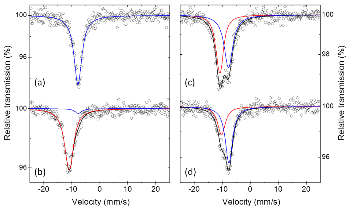
Figure 6. ^{121}\text{Sb} Mössbauer spectra at 78 K of Sb electrodes at the end of first discharge (a), at the end of first charge (b), after the reaction of 1.5 mol Na during first discharge (c) and after reaction of 2 mol Na during the first discharge (d).
