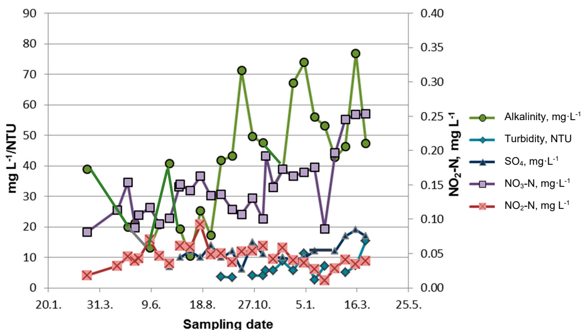
Figure 6. Measured parameters of water quality: alkalinity, NO 2 -N, NO 3 -N, SO 4 2- (mg·L -1 ), and turbidity (NTU) in RAS rearing rainbow trout ( Oncorhynchus mykiss ), and European whitefish ( Coregonus lavaretus ) over the course of the experiment.
