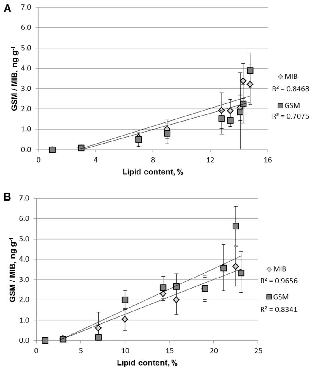
Figure 1. Concentrations of GSM and MIB ( \text{ng}\cdot\text{g}^{-1} , n = 4 , \pm SD) in European whitefish (A) and in rainbow trout (B) vs. lipid content in fish fillet (%) during the experiment.
