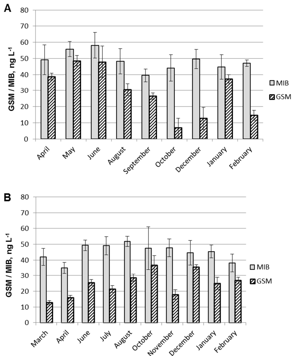
Figure 3. Concentrations of GSM and MIB ( \text{ng}\cdot\text{L}^{-1} , n = 4 , \pm SD) in circulating water for European whitefish ( A ) and rainbow trout ( B ) during the experiment.
