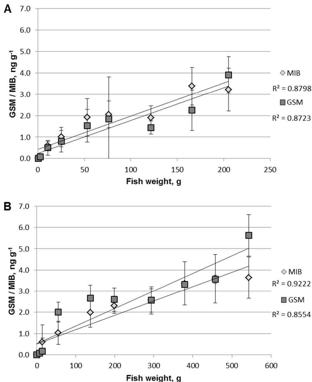
Figure 2. Concentrations of GSM and MIB (ng·g -1 , n = 4, ± SD) in European whitefish (A) and in rainbow trout (B) vs. weight (g) during the experiment.
