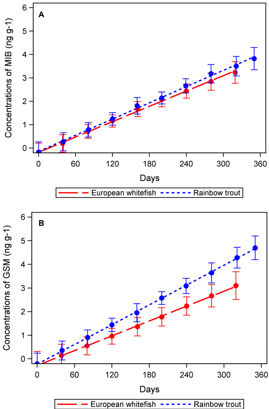
Figure 4. Increase of MIB (ng·g -1 , (A) and GSM concentrations (ng·g -1 , (B) vs. duration of experiment in days after every 40 days, based on the statistical model: rainbow trout (blue line) and European whitefish (red dashed line). Point estimates are shown with 95% confidence interval.
