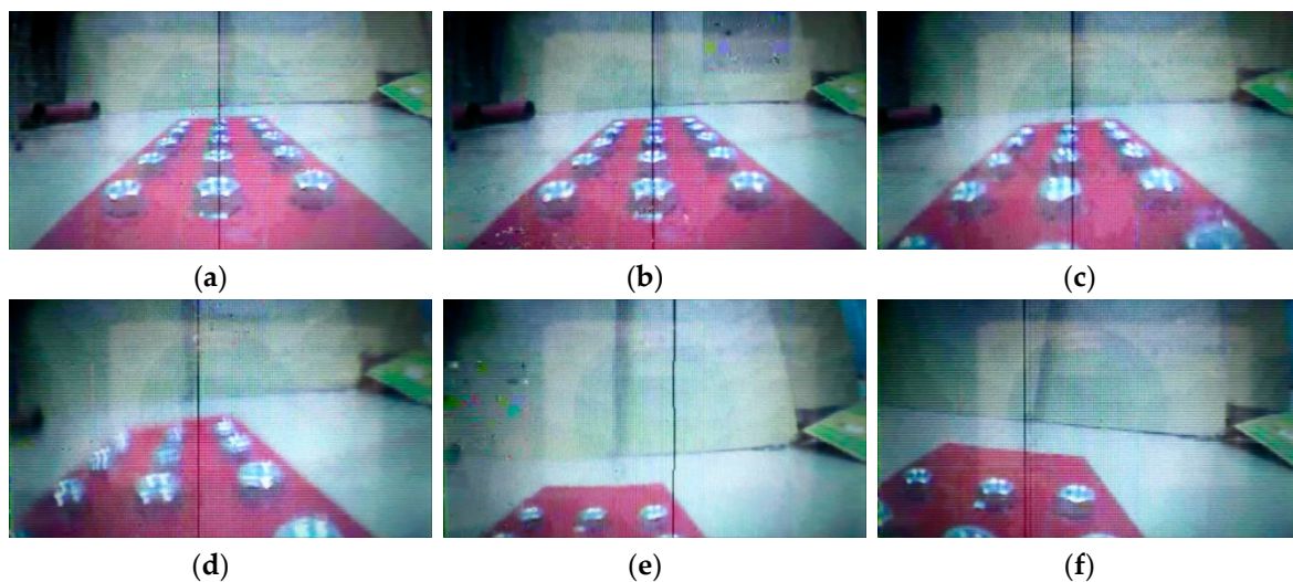
Figure 16. Images of camera attached to the front of BIREM without the control. (a) 0 s; (b) 1 s; (c) 2 s; (d) 3 s; (e) 4 s; (f) 5 s.
