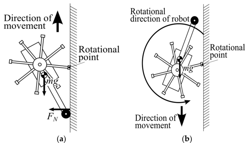
Figure 5. Attitude of the two-wheel-drive robot on the vertical wall. (a) Robot climbing wall; (b) robot moving down.
