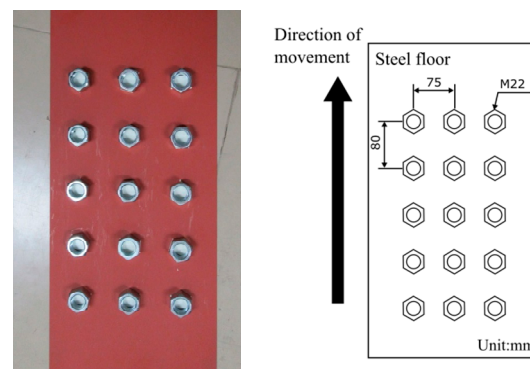
Figure 13. Model of the splicing part with 15 nuts for the experiment.
