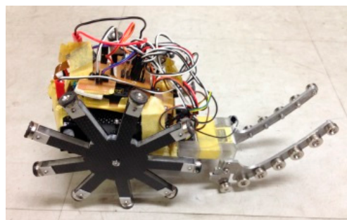
Figure 3. Bridge inspection robot (BIREM 3rd).
