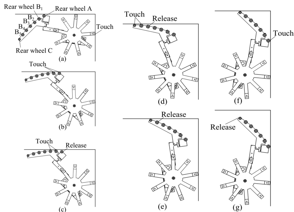
Figure 8. Robot running along the right-angled route. (a) Front wheel touches the vertical wall after the robot moving horizontally; (b) rear wheel B_1 touches the ceiling as well as the rear wheel A; (c) after rear wheel A released, rear wheel B_2 touches the ceiling promptly; (d) after rear wheel B_4 released, rear wheel C touches the ceiling promptly; (e) rear wheel B_5 is released from the ceiling; (f) while the rear wheel C is in contact with the ceiling, the rear wheel A contacts the vertical wall; (g) rear wheel C is released from the ceiling and the robot descends.
