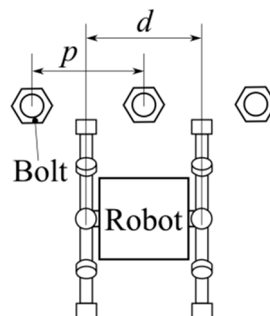
Figure 2. Bolt pitch of splice part. The length d is the wheel track of the robot and the length p is the interval of the bolts.
