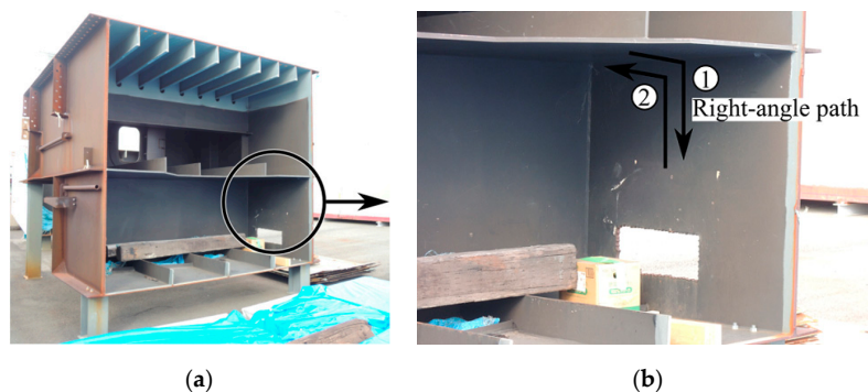
Figure 9. Box girder of the bridge. (a) External view; (b) enlarged view.
