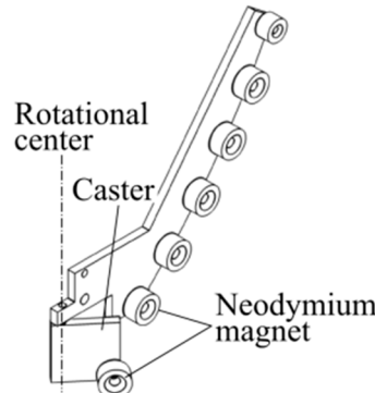
Figure 7. Magnetic rear wheels with a caster.
