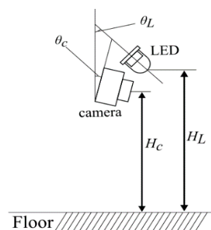
Figure 14. Position relationship between the camera and the LED attached to the robot.
