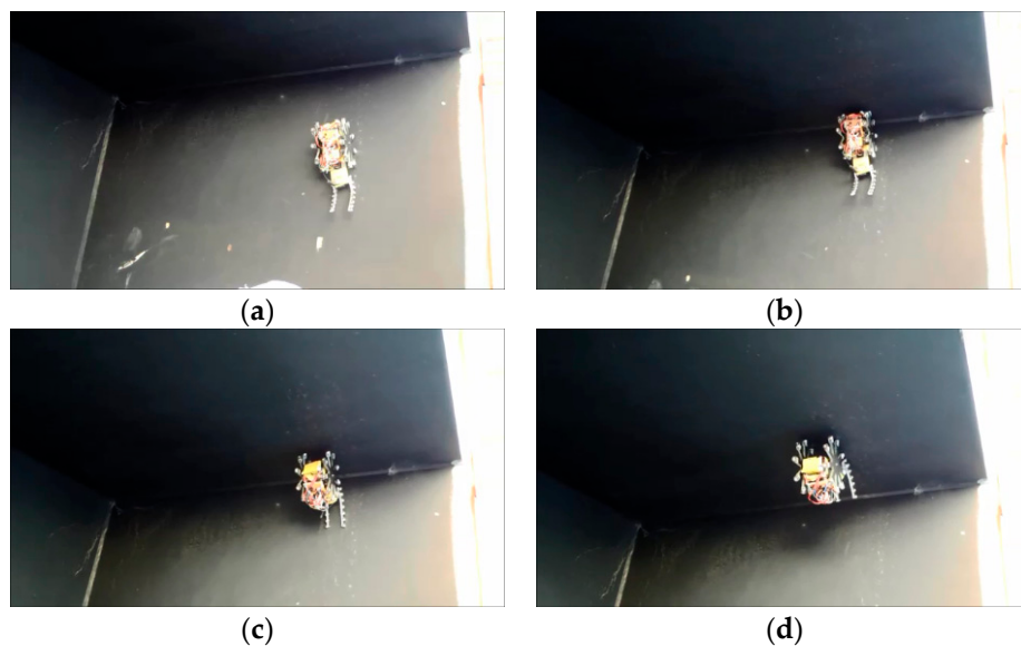
Figure 12. BIREM 3rd moving along route 2. (a) 0 s; (b) 3.3 s; (c) 6.7 s; (d) 10 s.
