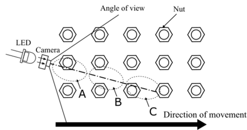
Figure 15. Position of each nut shown in the camera that changes based on the irradiation position of the LED (from A to C).
