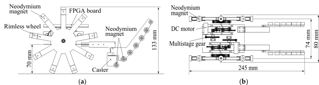
Figure 4. Mechanism of BIREM 3rd. (a) Side view; (b) top view.
