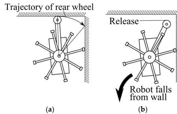
Figure 6. Robot falling from the right-angled route. (a) Rear wheel touching ceiling; (b) rear wheel releasing ceiling.
