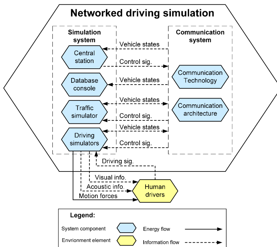
Figure 7. Example active structure partial model of a networked driving simulation system.
