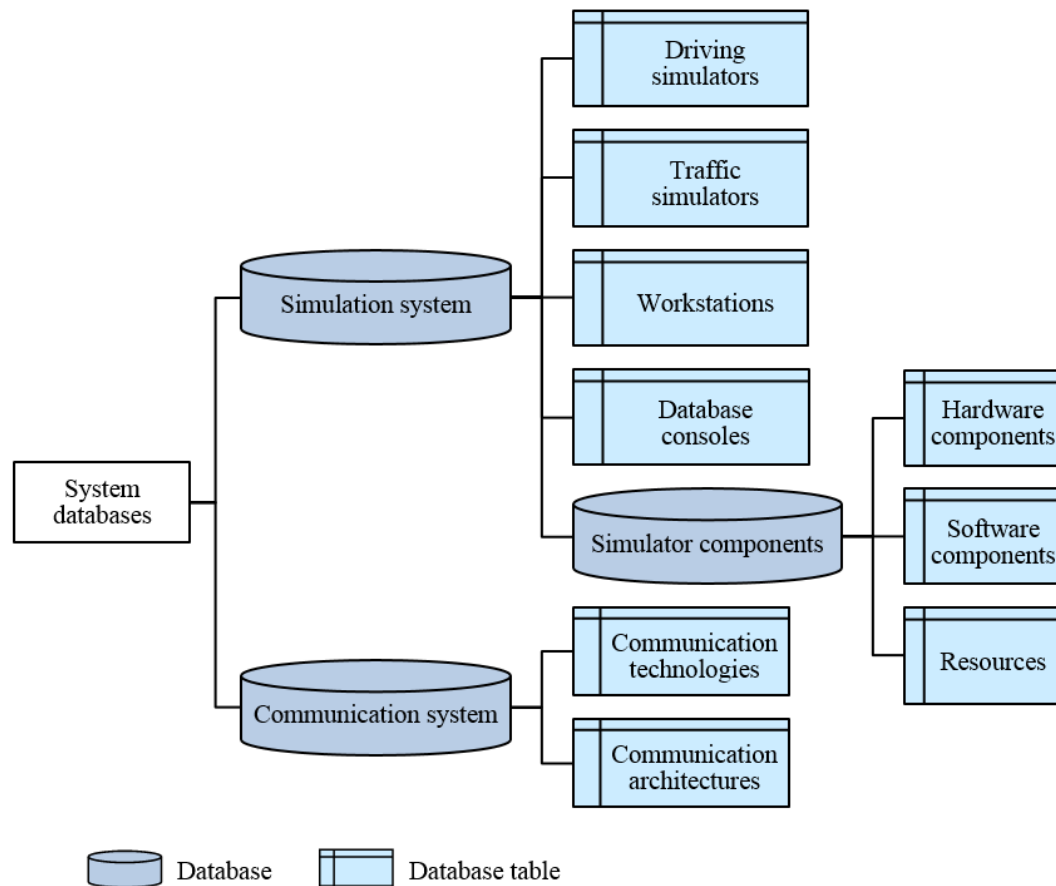
Figure 9. The developed system databases and the main tables.
