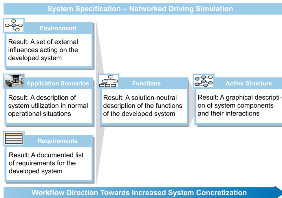
Figure 4. CONSENS workflow for networked driving simulation development.
