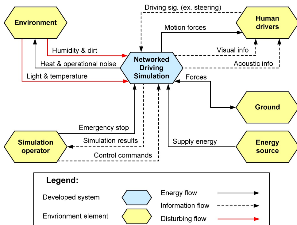
Figure 5. Example environment partial model of a networked driving simulation system.
