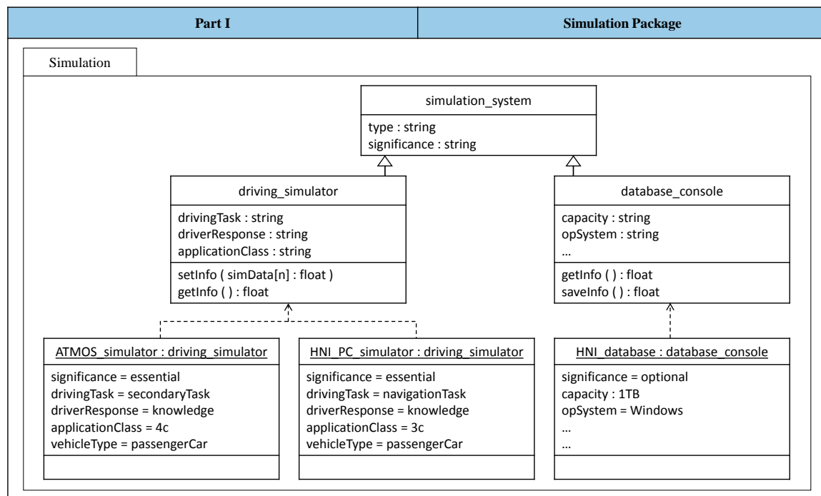
Figure 11. UML (The unified modeling language) class diagram of the selected simulation system components—package 1.
