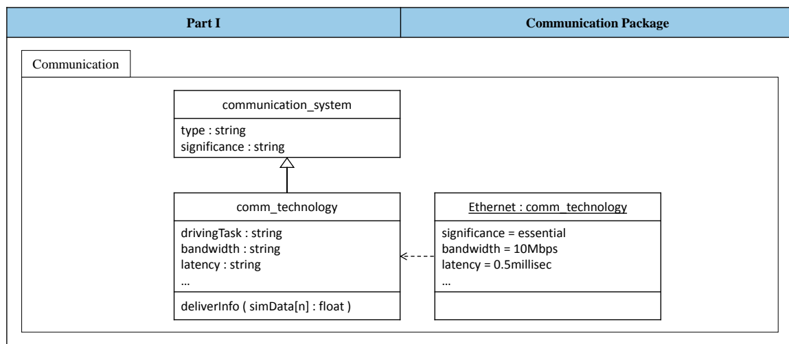
Figure 12. UML class diagram of the selected communication system components—package 2.
