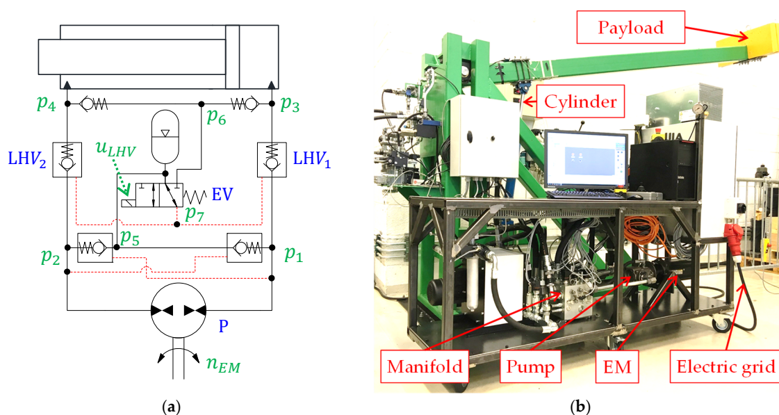
Figure 1. (a) Simplified schematic of the self-contained cylinder; (b) the experimental setup.
