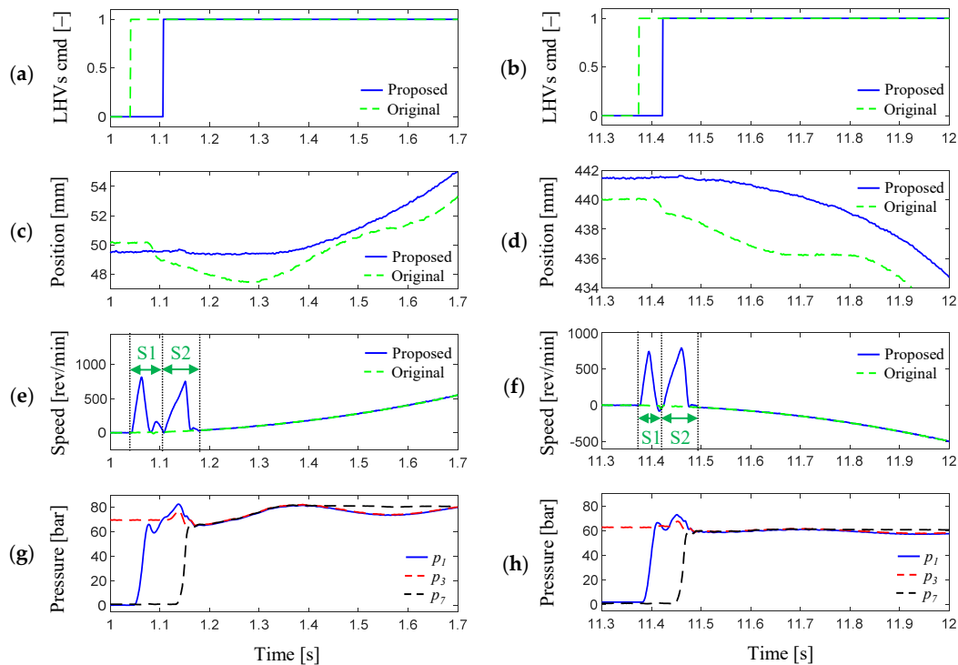
Figure 4. A representative working cycle: (a,b) load-holding valve's commands; (c,d) measured piston positions; (e,f) measured EM's speeds; (g,h) measured pressures.
