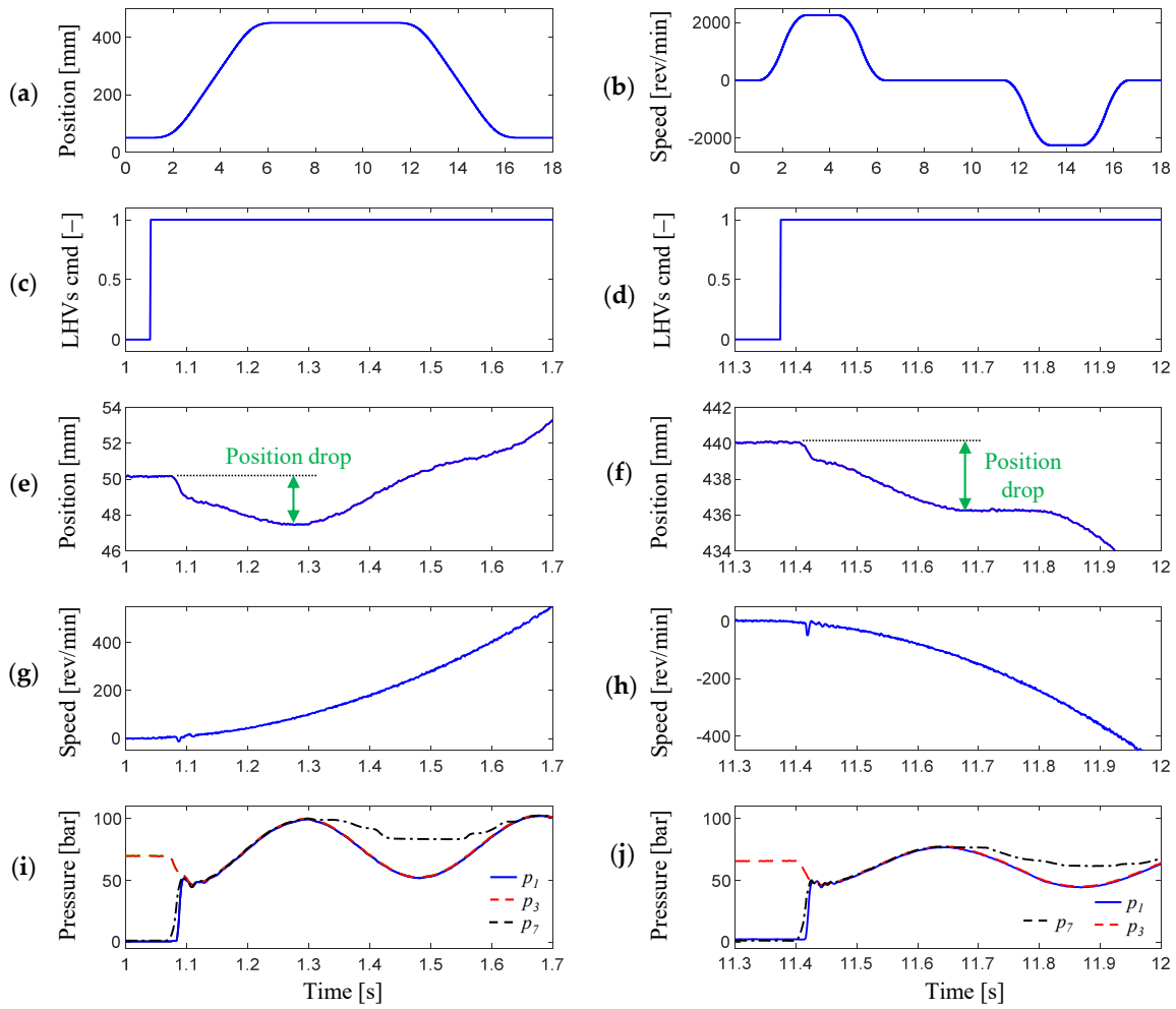
Figure 2. A representative working cycle: (a) desired piston position; (b) resulting electric motor's (EM) speed command; (c,d) load-holding valve's command; (e,f) measured piston position; (g,h) measured EM's speed; (i,j) measured pressures.
