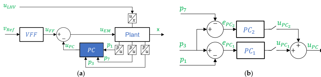
Figure 3. (a) Proposed control structure of the self-contained cylinder for open-loop position control; (b) detail of the pressure controller.
