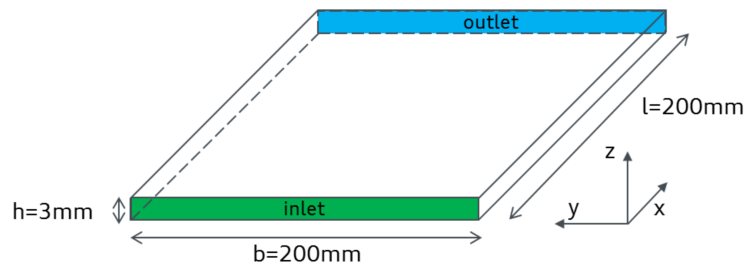
Figure 2. Simulation model used for verification with inlet and outlet boundary conditions.
