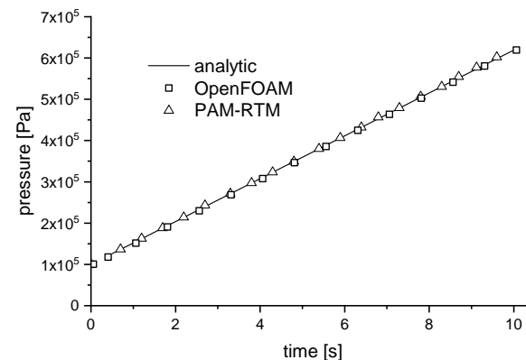
Figure 5. Pressure increase at the inlet while Injection-RTM boundary conditions are applied.
