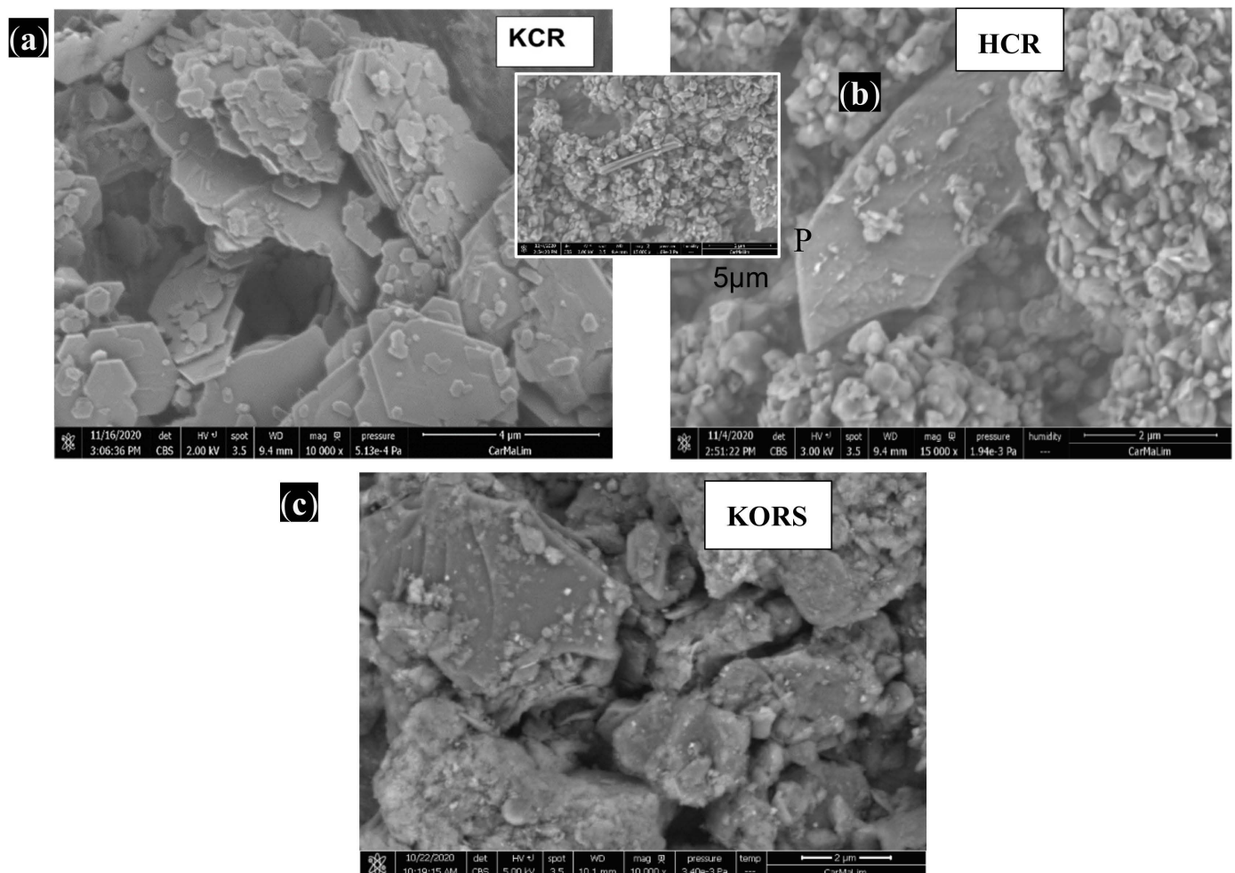
Figure 3. SEM images of particle morphology of (a) KCR, (b) HCR, and (c) KORS powders. P = Primary mullite.
