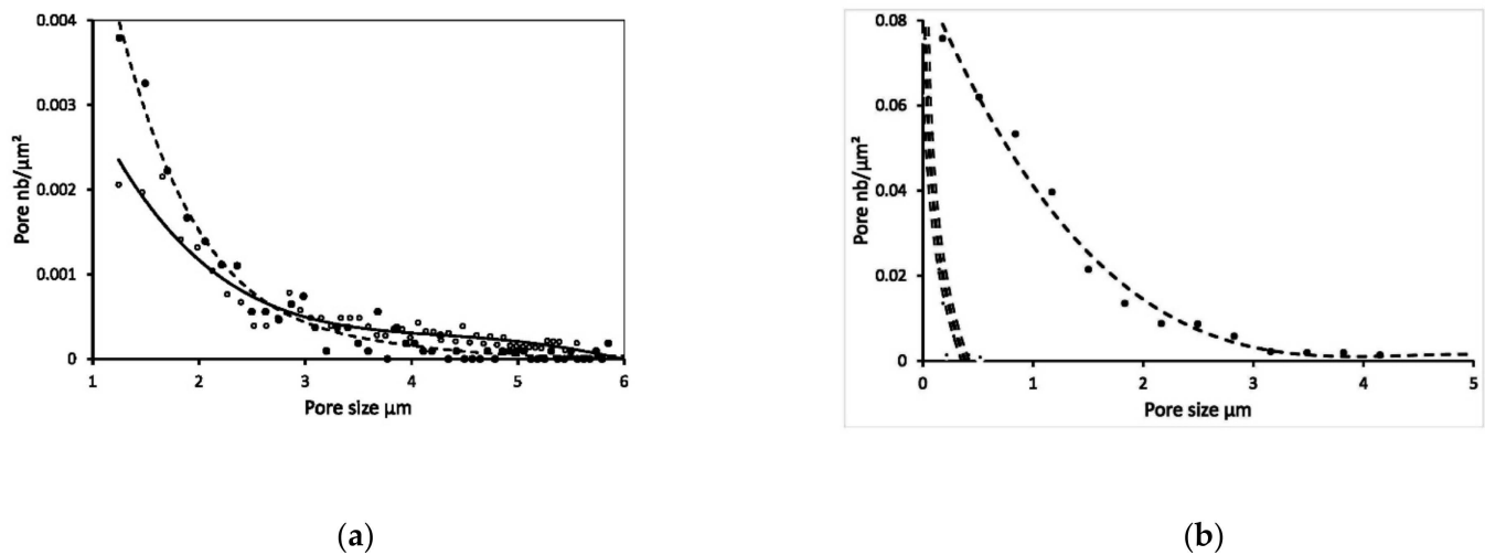
Figure 12. (a) Pore numbers per \mu\text{m}^2 of HCR (●) and KORS (o) against the pore size; (b) Grain (●) and pore numbers (thick line) of KCR per \mu\text{m}^2 against the grain and pore sizes.
