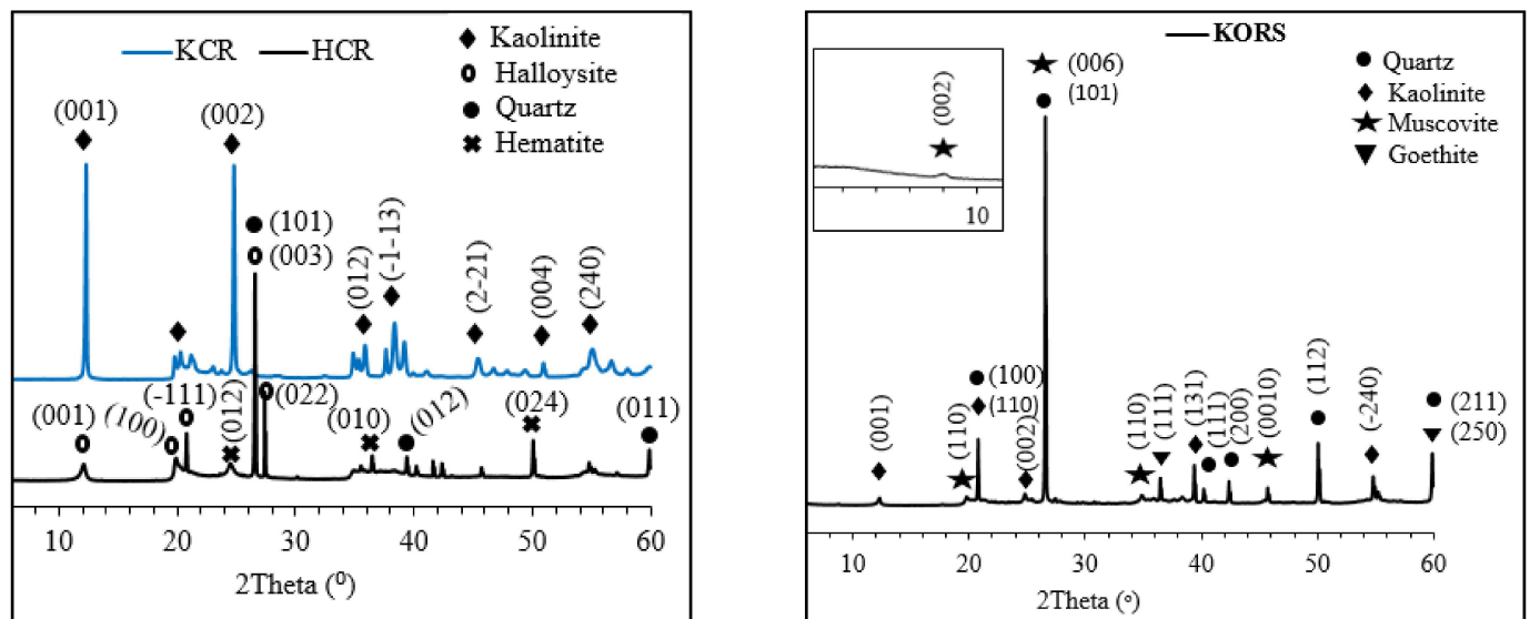
Figure 2. XRD patterns of raw materials.
