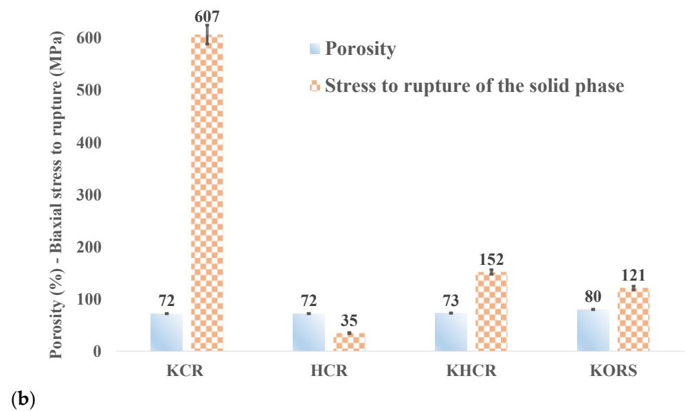
Figure 8. Biaxial flexural strength and porosity of (a) manufactured porous ceramics and (b) corresponding solid-phase stress-to-rupture. Discs sintered at 1200 °C.
