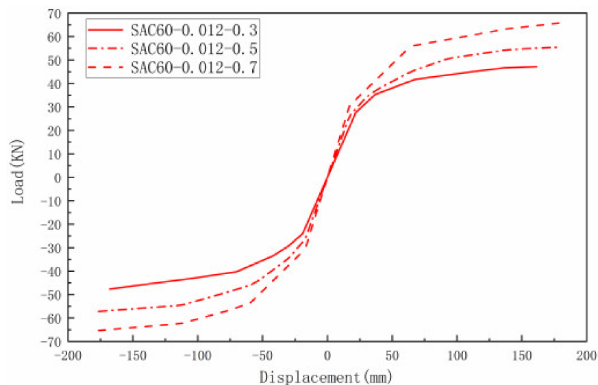
Figure 18. Skeleton curves of specimens.
