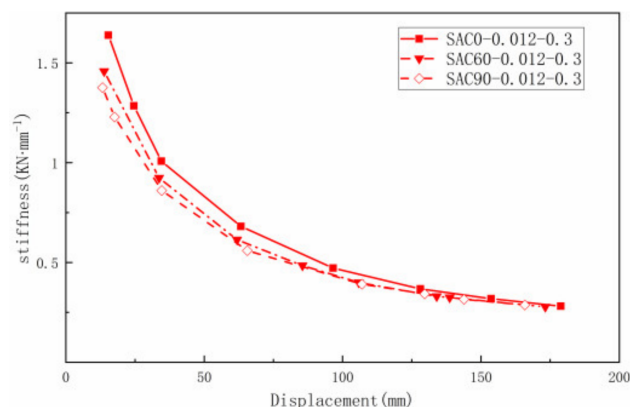
Figure 10. Relationship between stiffness degradation and displacement.
