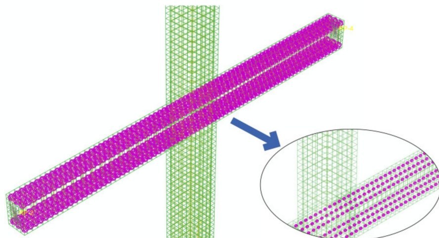
Figure 6. Spring cell setting.
