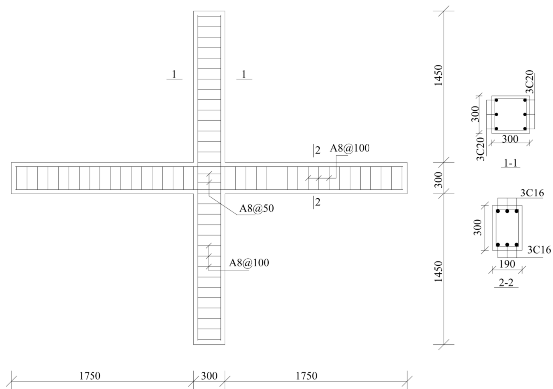
Figure 7. Dimensions and reinforcement of SAC beam-column joints.
