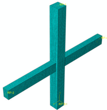
Figure 5. Grid division.
