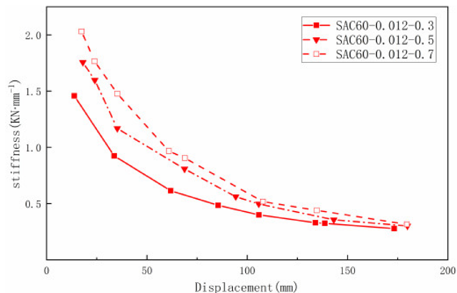
Figure 19. Relationship between stiffness degradation and displacement.
