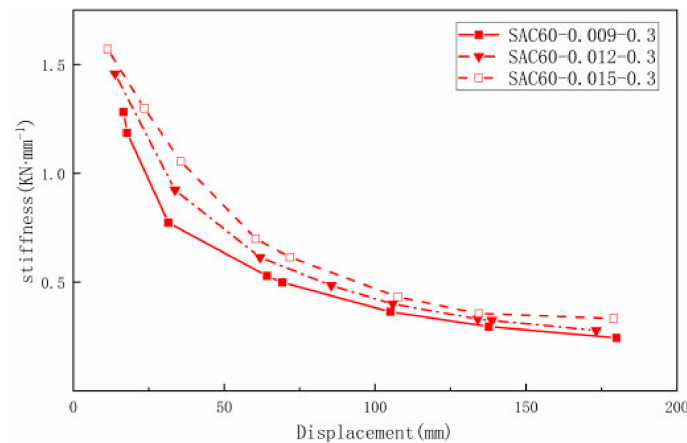
Figure 16. Relationship between stiffness degradation and displacement.
