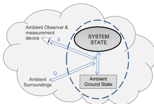
Figure 1. Perfect measurement is a reversible transformation from a system's initial state to its ambient ground state reference. Perfect reversible measurement involves transfers of exergy ( X ) and ambient heat ( Q ) to the surroundings. Reversing the process restores the system's initial pre-measurement state.
