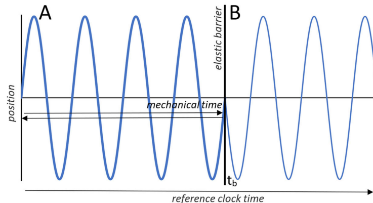
Figure 3. Mechanical and reference times. (A) Plot shows the trajectory of a one-dimensional harmonic oscillator over parallel advances in mechanical and reference times. (B) Mechanical and reference times decouple when the oscillator encounters an elastic barrier momentarily inserted at time t_b . The oscillator and mechanical time, as an index of the oscillator's position, reverse direction and retrace the trajectory over mechanical time. The trajectory in B shows the oscillator's position across reference time, which continues to advance without bound.
