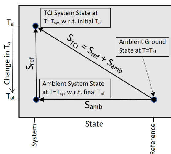
Figure 2. The two components of TCI entropy.
