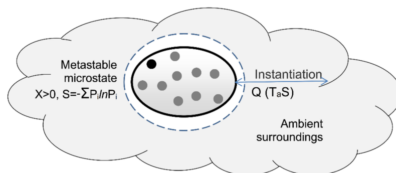
Figure 5. Instantiation of metastable microstate. The microstate initially has positive entropy and comprises multiple measurable potentialities (dots). Instantiation involves the transfer of ambient heat and entropy to the surroundings. This reduces the microstate's entropy to zero and randomly instantiates a single zero-entropy potentiality (black dot).
