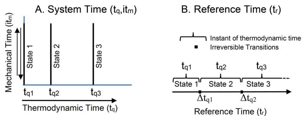
Figure 4. Complex system time and reference time. (A) Shows the complex system time plane, spanned by real-valued thermodynamic time (horizontal axis) and imaginary mechanical time (vertical axis). (B) Shows the irreversible advance in reference time over reversible intervals of system time at a fixed thermodynamic time, t_{qi} , and between irreversible transitions over intervals of thermodynamic time, \Delta t_{qi} .
