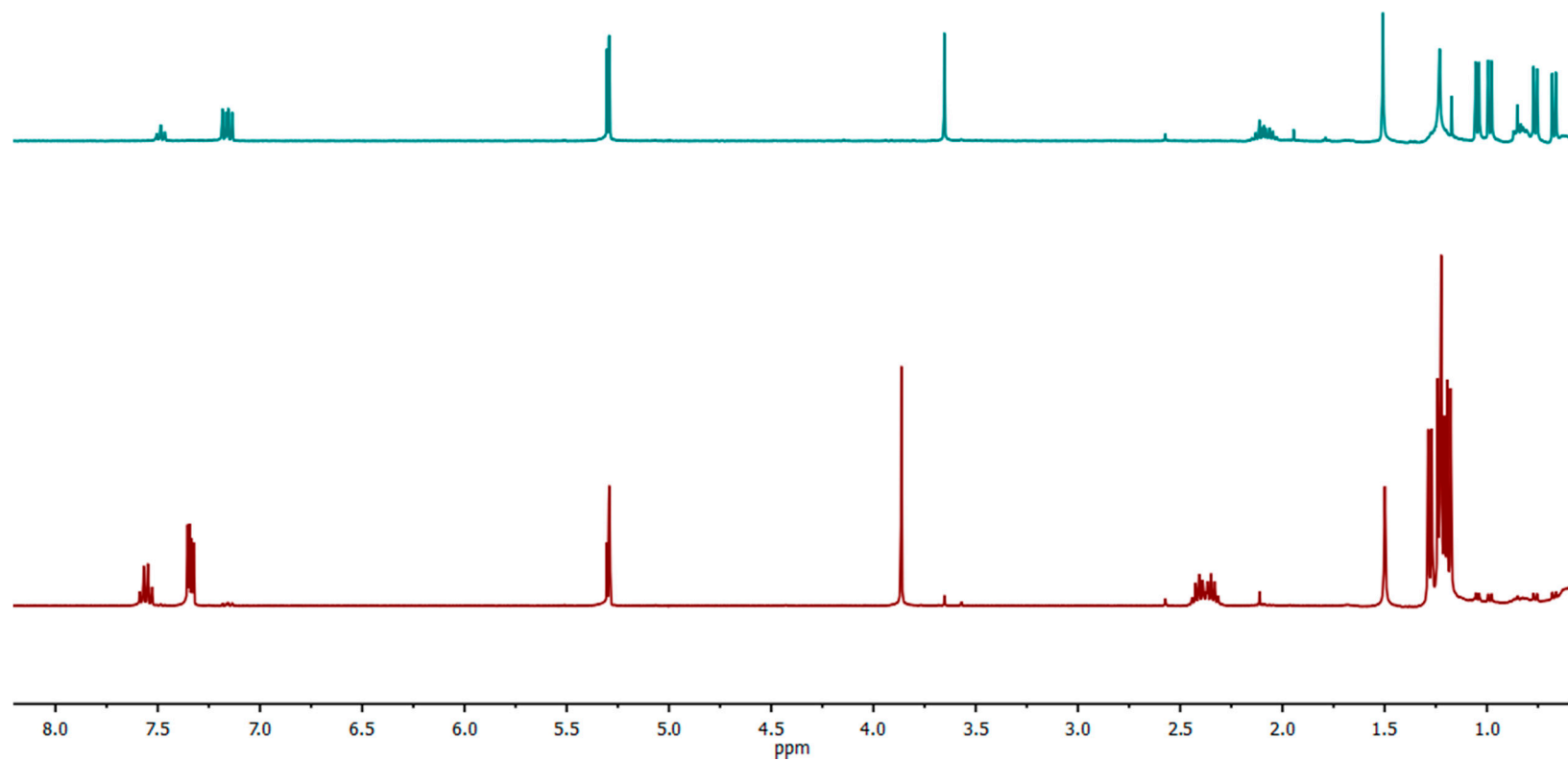
Figure S2. Stacked ^1\text{H} -NMR spectra of 1b (red line) and 2b (blue line).
