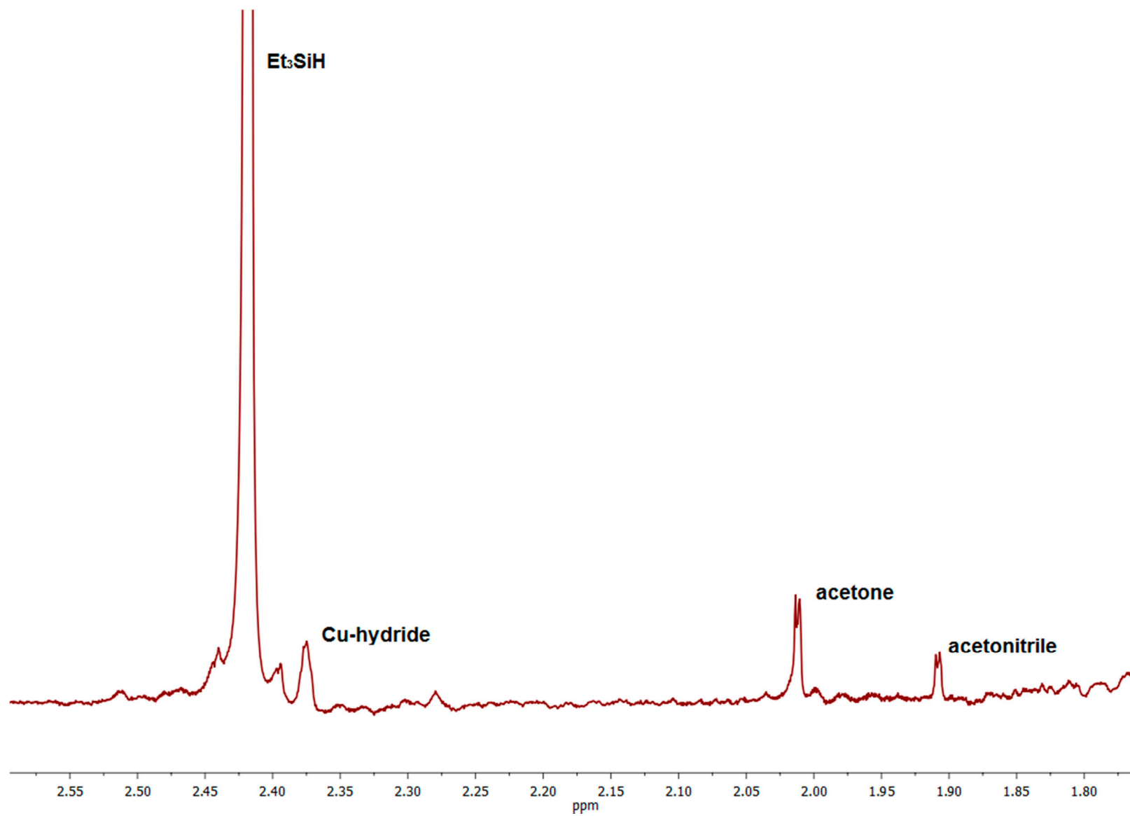
Figure S3. Potential hydride signal from the reaction of 1c with Et 3 SiH.
