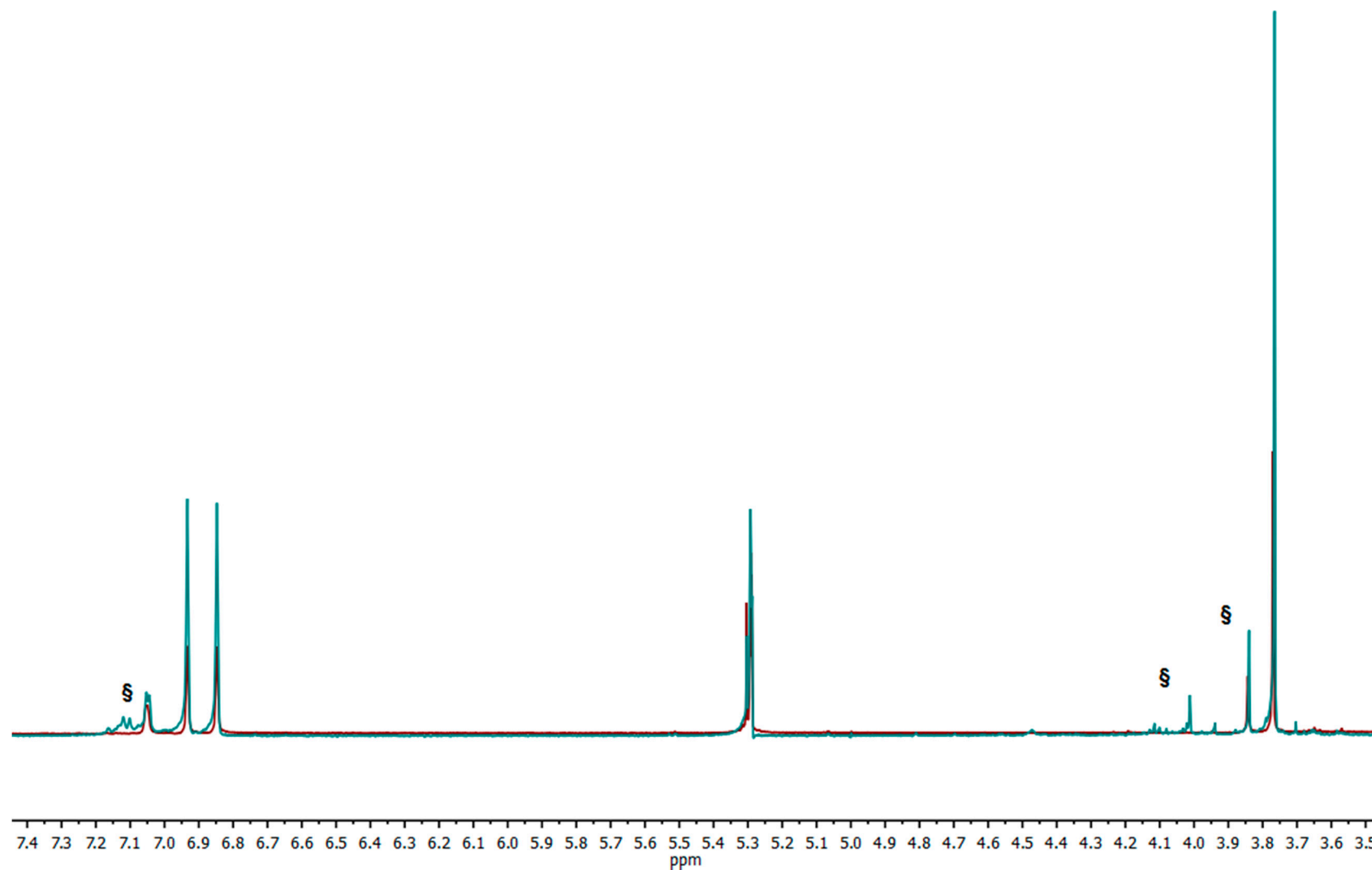
Figure S1. Superimposed ^1\text{H} -NMR spectra of 2a (red line) and 2a (blue line); § indicates small decomposition byproducts.
