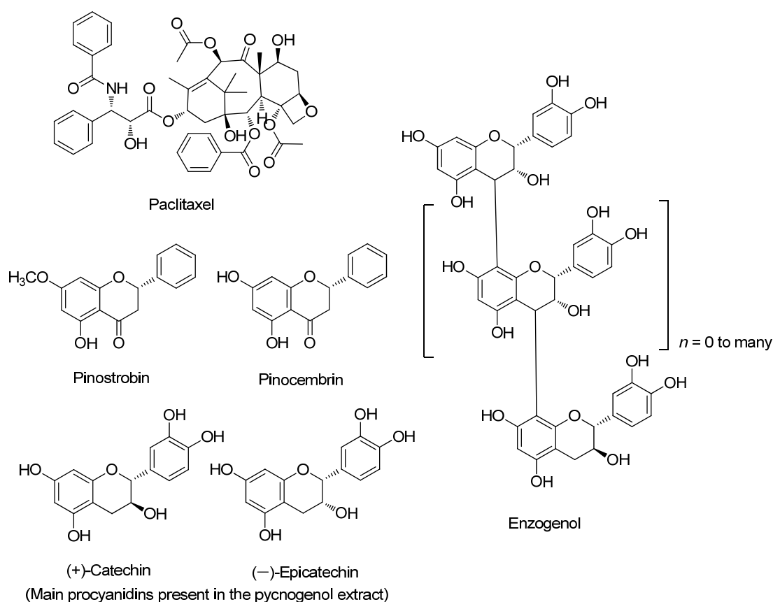
Figure 1. Chemical structures of the commercially available products displayed in Table 1.
