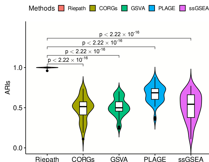
Figure 1. Hierarchical clustering comparison measured by ARI index.
