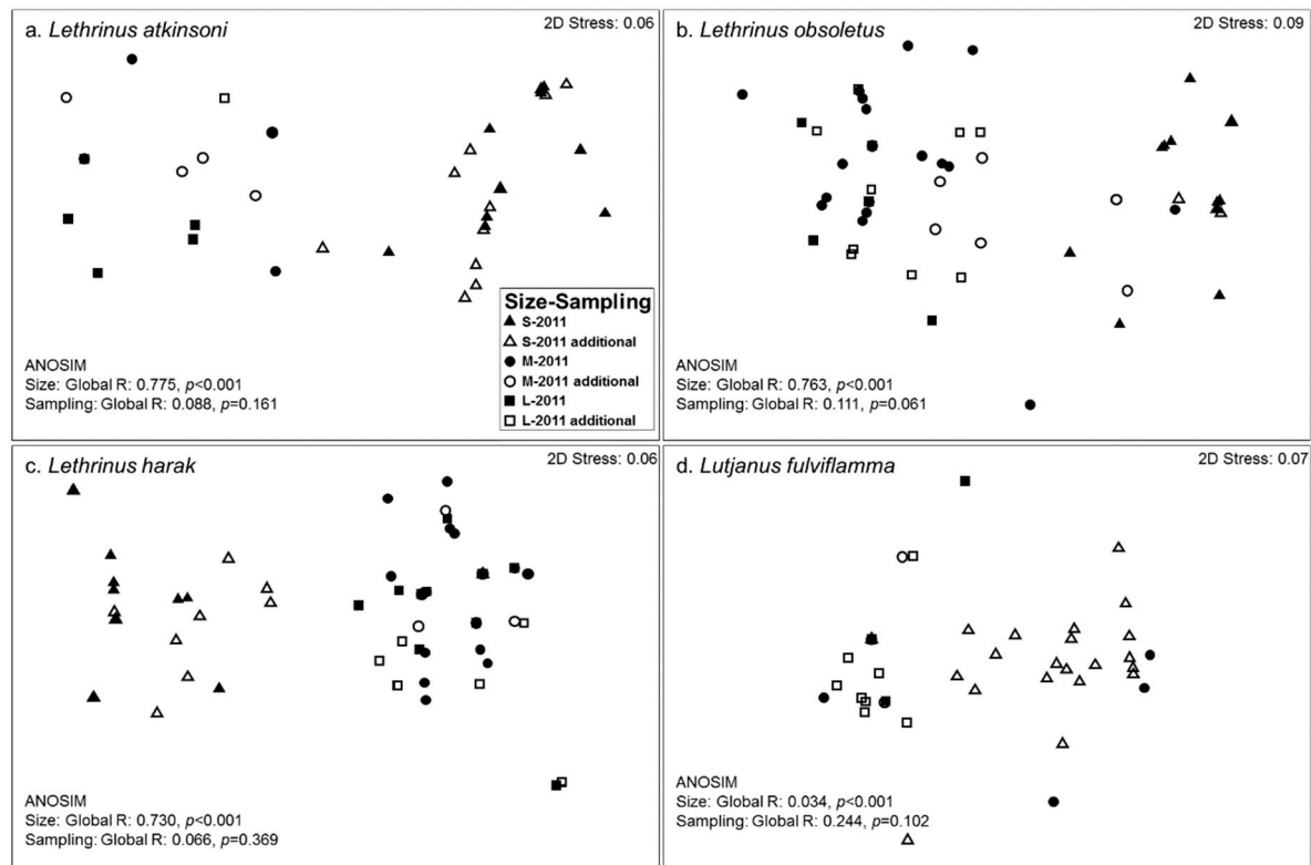
Supplemental material Figure S1. MDS results of stomach content analysis form previous study and additional sampling of (a) Lethrinus atkinsoni ; (b) Lethrinus obsoletus ; (c) Lethrinus harak and (d) Lutjanus fulviflamma . All data show significant different between body size, but was not significant different between two sampling. The abbreviations of body length size categories are S: small, M: medium and L: large.
