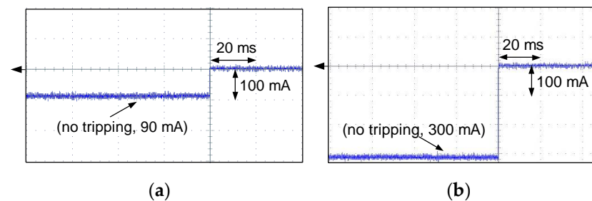
Figure 28. Oscillograms of the DC current flow during NO tripping of the F-type RCD (RCD30_5). Suddenly applied DC current of the following values: (a) 90 mA; (b) 300 mA.
