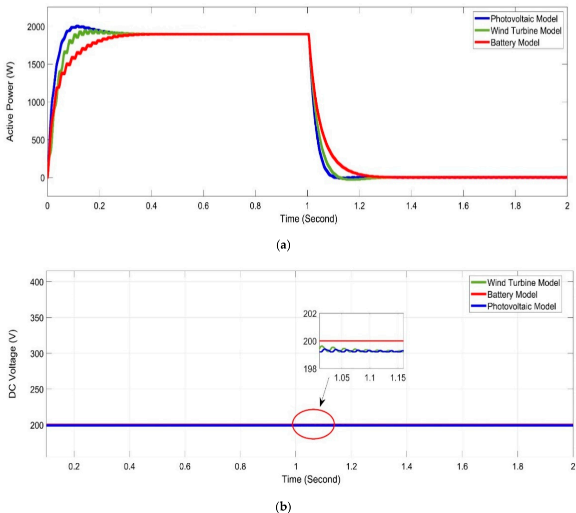
Figure 12. Simulation of identical distribution lines are used, (a) inverters power response, (b) DC link voltage response under loads change.
