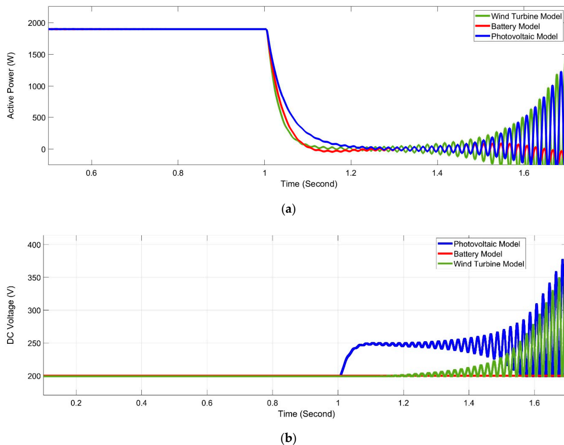
Figure 20. Simulation result, where (a) the averaged power response, (b) response of DC link voltage.
