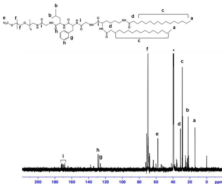
Figure S1. 13 C-NMR spectrum of PEG-GLFG in DMSO-d 6 (600MHz).
