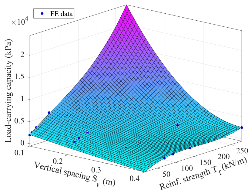
Figure 13. Relation between load-carrying capacity, reinforcement strength, and reinforcement spacing of the study GRS mass.
