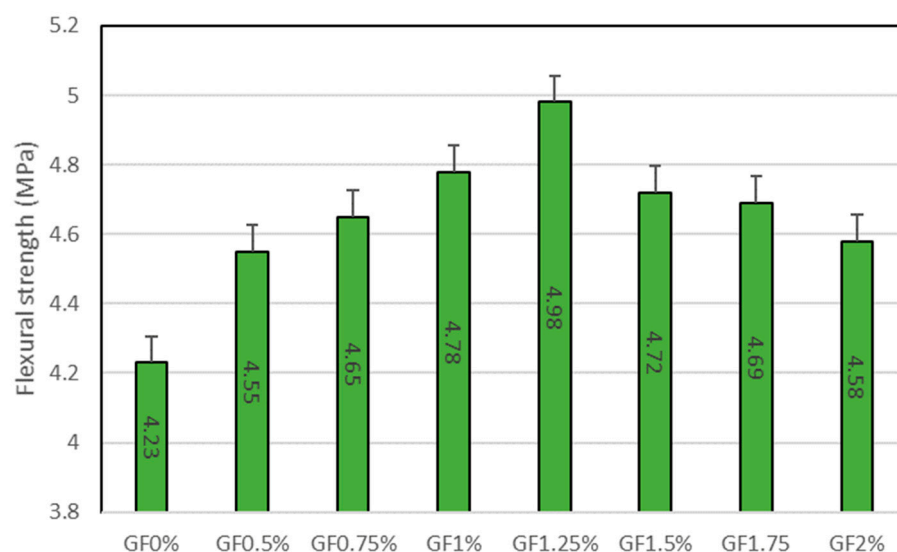
Figure 5. Flexural strength.
