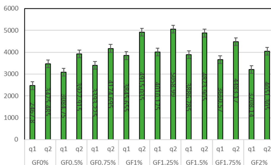
Figure 7. Impact Energy.
