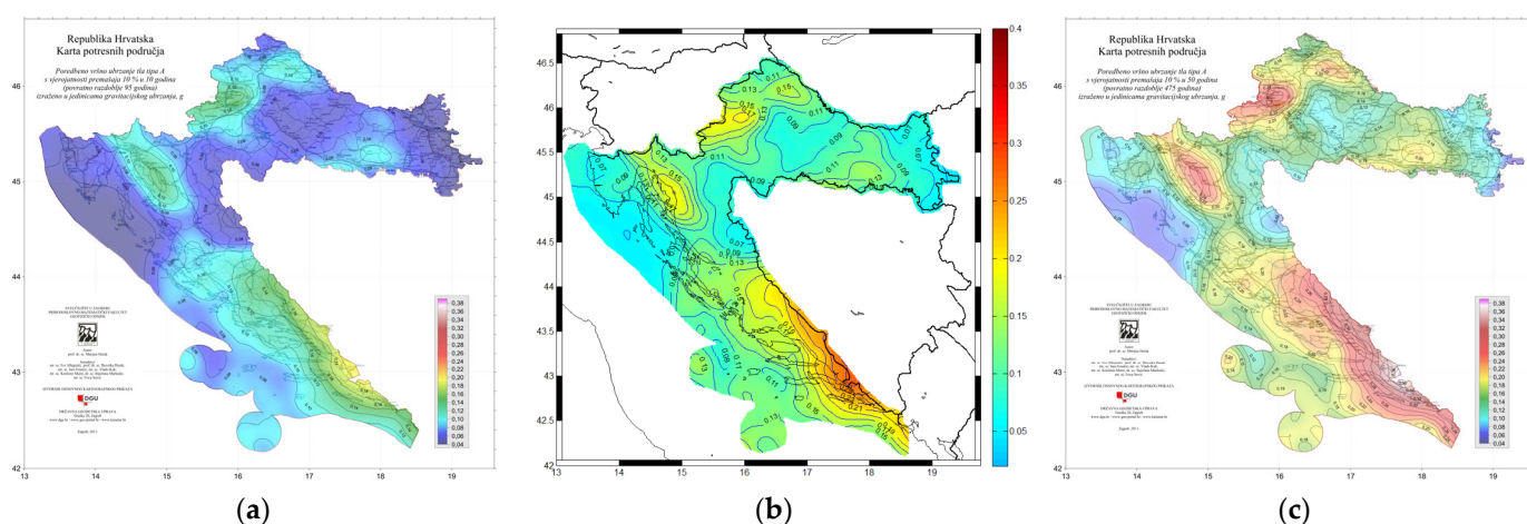
Figure 21. The Earthquake Hazard Maps of the Republic of Croatia for the return period of (a) 95, (b) 225, and (c) 475 years (publicly available at URL: http://seizkarta.gfz.hr/hazmap/karta.php ; accessed on 22 September 2023).
