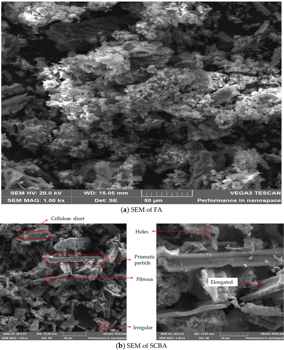
Figure 2. SEM picture of (a) FA and (b) Processed SCBA.
