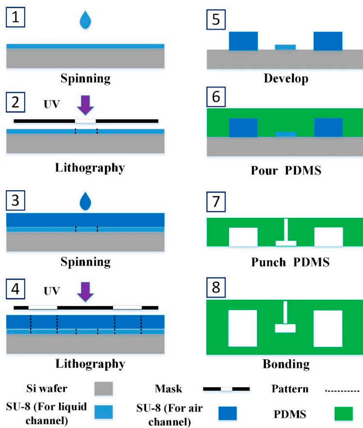
Figure S1. Fabrication process of the 3D ESFFI microfluidic chip.
