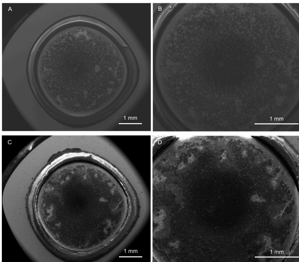
Figure S1. SEM micrographs at different magnifications of \text{Mn}_x\text{O}_{1+x} films on RDE before (A,B) and after (C,D) ADT cycling (5000 cycles at 50 \text{ mV}\cdot\text{s}^{-1} between 0.4 and 0.8 V vs. Ag/AgCl, in a 0.5 M \text{H}_2\text{SO}_4 solution).
