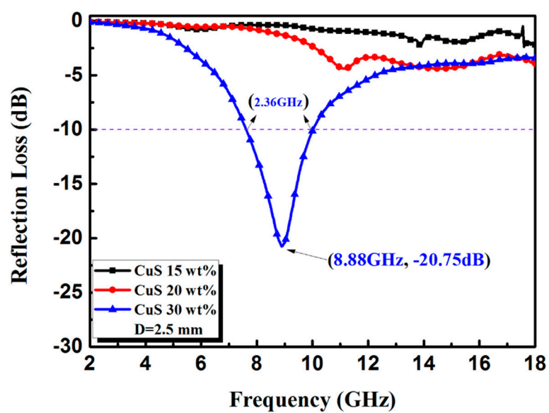
Figure S2. Reflection loss curves of paraffin composites containing 15 wt% 20 wt% and 30 wt% CuS under the thickness of 2.5 mm.
