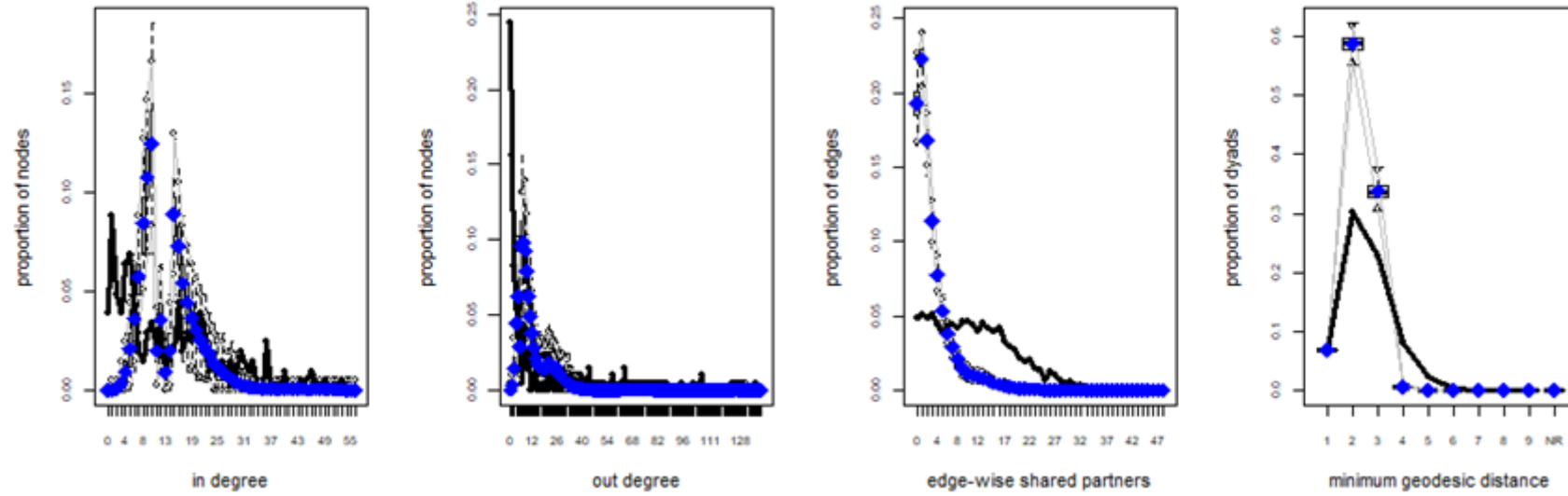
(b) Goodness of fit diagnostic for ERGM-WTN (2014-2018)
