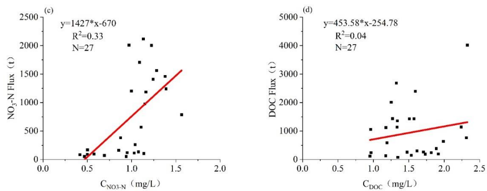
Fig. S3 Scatter plots show the mean monthly water quality and monthly nutrient flux by measurements
