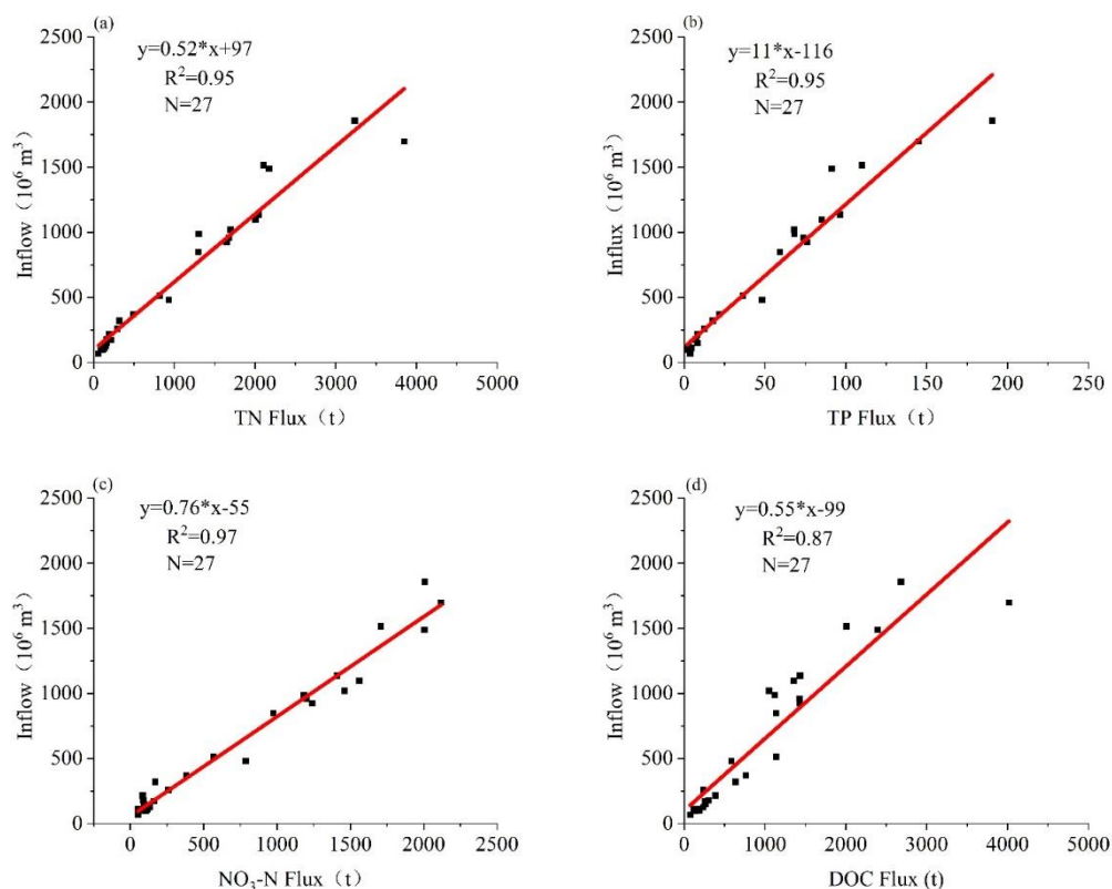
Fig. S2 Scatter plots show the monthly inflow and monthly nutrient flux by measurements
