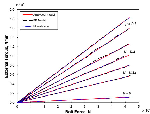
Figure 8. Torque and bolt force in M12 \times 1.75 bolt for different friction coefficients.
