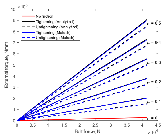
Figure 9. Comparison of analytical and Motosh models with torque and bolt force in M36 \times 4 bolt for different friction coefficients.
