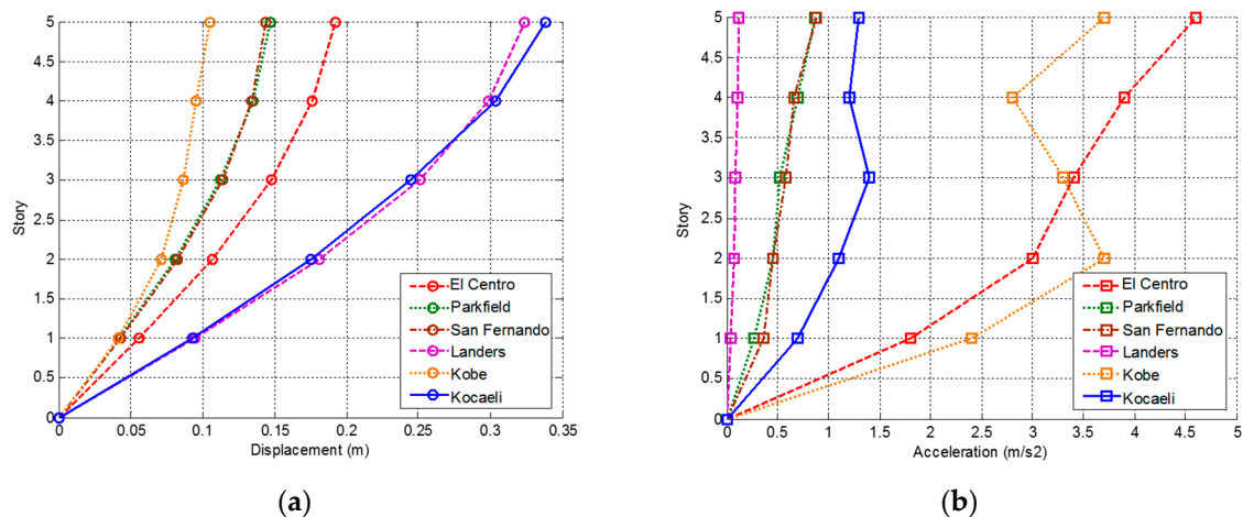
Figure 5. The results of (a) peak displacement and (b) peak acceleration for different stories of building after changing the story stiffness.
