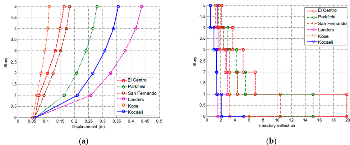
Figure 16. The results of (a) peak displacement and (b) peak interstory deflection for different stories of isolated buildings with rubber bumpers.
