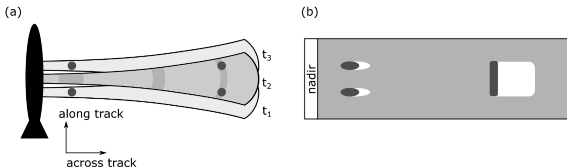
Figure 5. Along track object detection is depending on the across track distance (ground range). Closely spaced objects far from the nadir are imaged as one object due to beam spreading (modified after Blondel and Lurton [84]). (a) Horizontal beam evolution and size of footprint in relation to the across track distance for time stamp t : 1–3. (b) Schematic sonar image.
