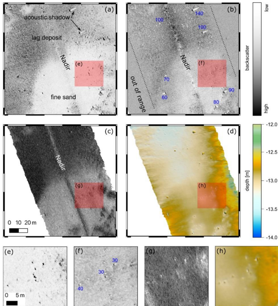
Figure 2. Backscatter and bathymetry data of a hard-substrate area: (a) 400 kHz SSS, (b) 900 kHz SSS, (c) MBES 300 kHz, (d) MBES bathymetry. Red boxes represent insets of (e–h). Data resolution is 25 cm. The blue numbers indicate the calculated object height in centimeters. SSS height above the sea floor was approximately 6.5 m.
