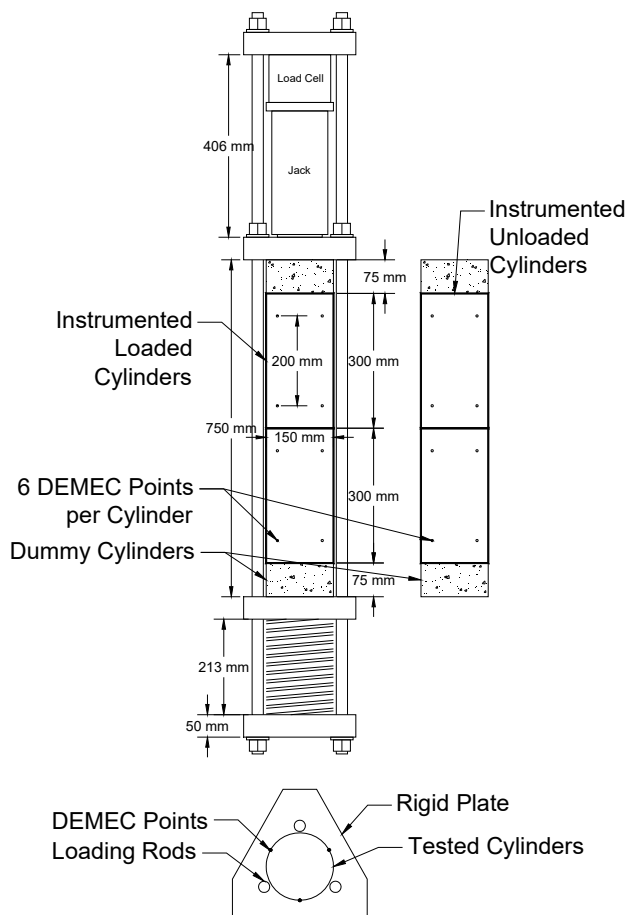
Figure 3. Creep test setup and specimen dimensions (25 mm = 1 in.).
