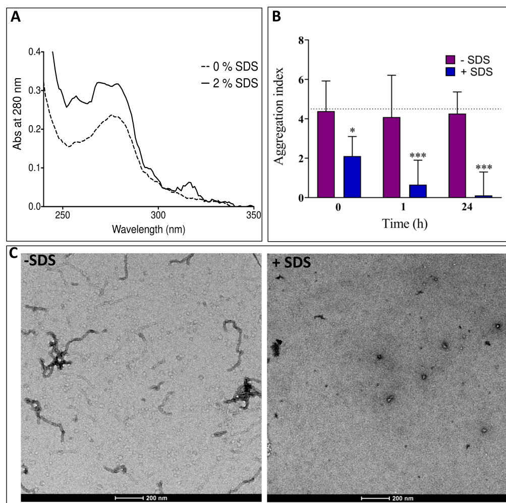
Figure 9. (A) Absorbance at 280 nm of the filtrate of a sample of PNT3 at 100 \mu M after 56 h of incubation at 37 °C before (dashed line) and after (continuous line) exposure to 2% SDS, and 10 min incubation at 37 °C. Exposure of SDS enables more material to pass through the filter. (B) Aggregation index of a fibrillated sample of PNT3 at 100 \mu M before and after incubation at RT either in the presence or in the absence of 2% SDS. Exposure to SDS reduces the aggregation index. The error bar corresponds to the standard deviation with n = 5 . The asterisks denote a statistically significant difference with respect to the sample without SDS (* p < 0.0265 ; *** p < 0.0004 , one-way ANOVA test). (C) Micrographs of a PNT3 sample at 200 \mu M after 56 h of incubation at 37 °C either in the absence or in the presence of 5 mM (1.44 mg mL -1 ) SDS.
