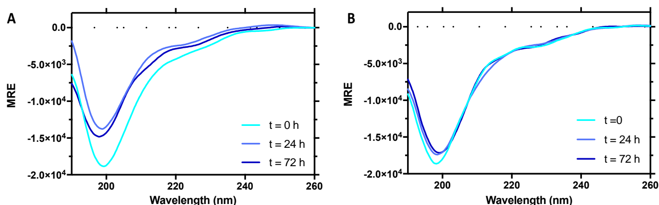
Figure 5. Far-UV circular dichroism (CD) studies of PNT3 (A) and PNT3 3A (B). The spectra were recorded in 10 mM sodium phosphate pH 6.5 at 37 °C. Protein concentration was at 0.06 mg mL −1 (4 μM). The spectra shown in cyan correspond to a freshly purified PNT3 or PNT3 3A sample recorded immediately after elution from the SEC column. The spectra shown in light and dark blue were recorded from the same samples incubated at 37 °C for 24 h and 72 h, respectively. Note the much more pronounced decrease in the signal for the spectrum at 24 h of PNT3 compared to PNT3 3A . MRE (Θ) is expressed in deg cm 2 dmol −1 .
