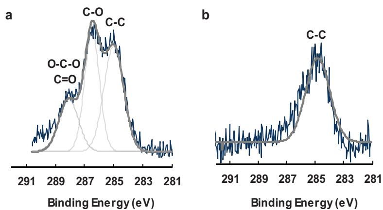
Figure S2. High-resolution XPS spectra of (a) GlcNAc6-immobilized and (b) GlcNAc6-free Au surfaces.
