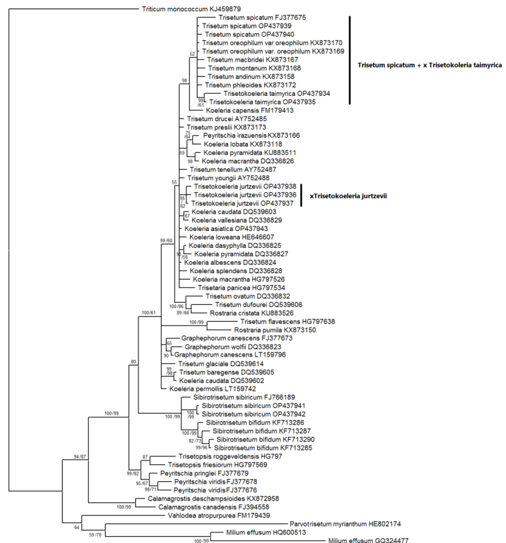
Figure 6. Phylogenetic tree of the genus xTrisetokoeleria and related species according to the ITS sequence data. The first index on the branch is the posterior probability in Bayesian inference, the second is the bootstrap index obtained by Maximum Likelihood algorithm. When only one index is shown on the branch it is the posterior probability.
