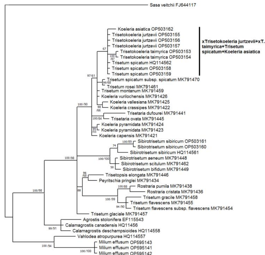
Figure 5. Phylogenetic tree of the genus xTrisetokoeleria and related species according to the trnK–rps16 sequence data. The first index on the branch is the posterior probability in Bayesian inference, the second is the bootstrap index obtained by Maximum Likelihood algorithm. When only one index is shown on the branch it is the posterior probability.
