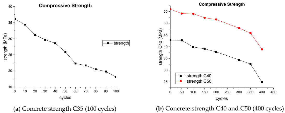
Figure 7. Compressive strength changes of concrete samples in association with freeze–thaw cycles.
