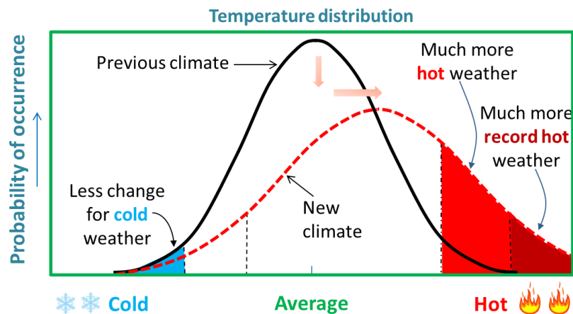
Figure 3. The temperature change between previous years and recent years [1].
