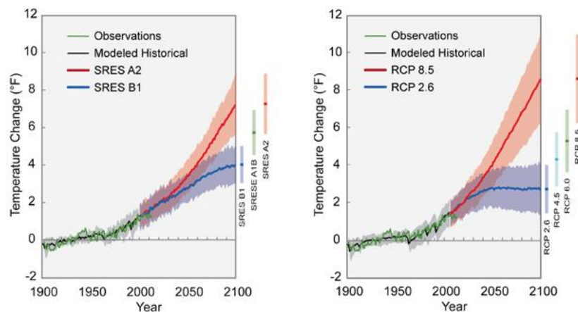
Figure 5. Emissions and temperature [28].
