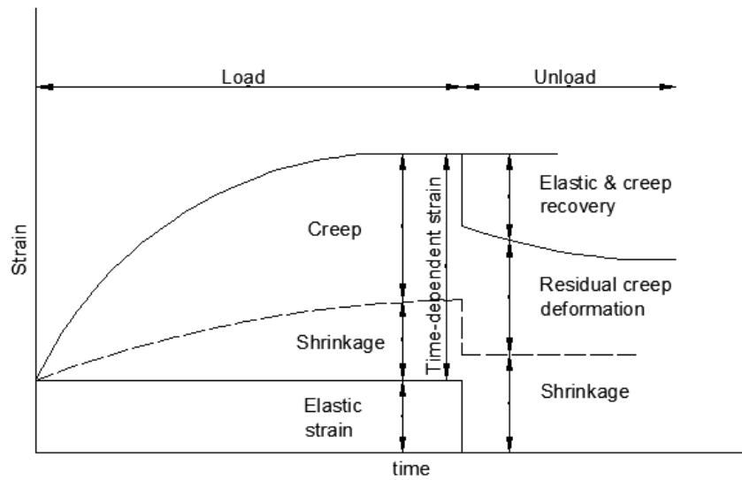
Figure 6. Creep strain after loading.
