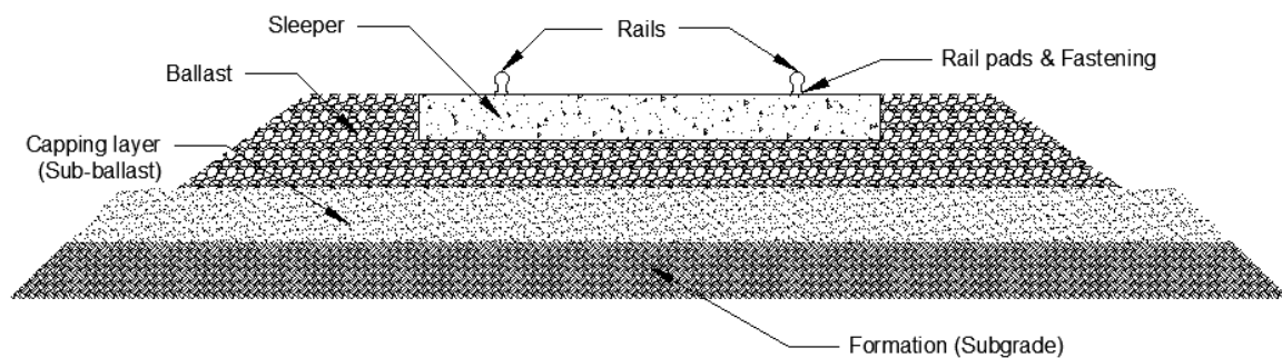
Figure 2. Conventional railway structure.
