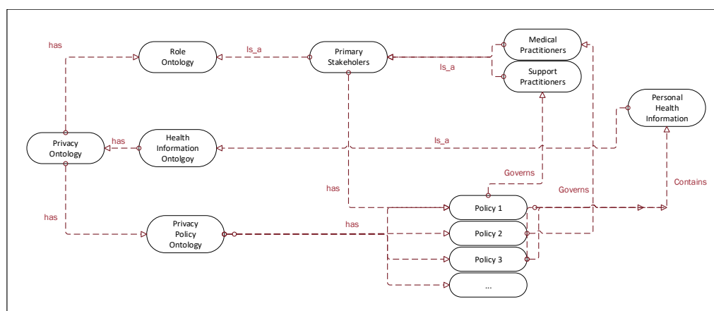
Figure 5. Privacy policy ontology.
