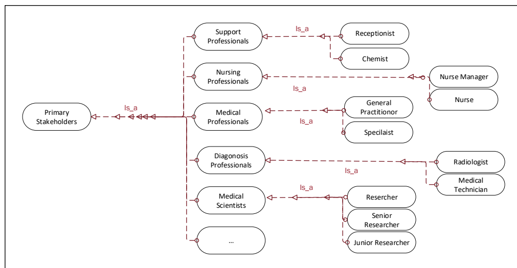
Figure 3. Role ontology.
